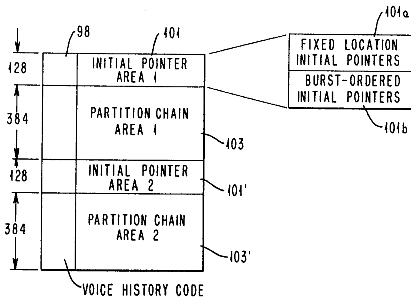
FIG. 15 BURST PRIORITY RAM 100
