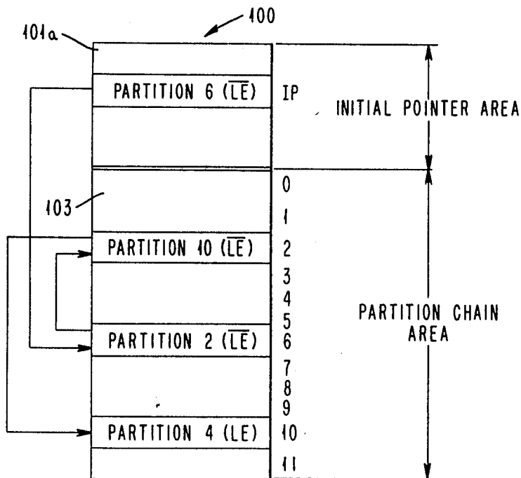
FIG. 16 TRANSMIT LIST STRUCTURE IN BURST PRIORITY RAM
