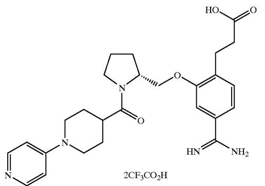
Compound of Example 26
