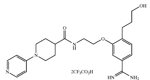
Compound of Example 43
