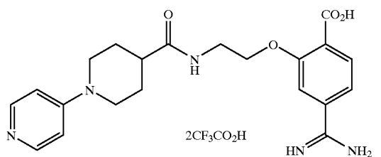
Compound of Example 37
