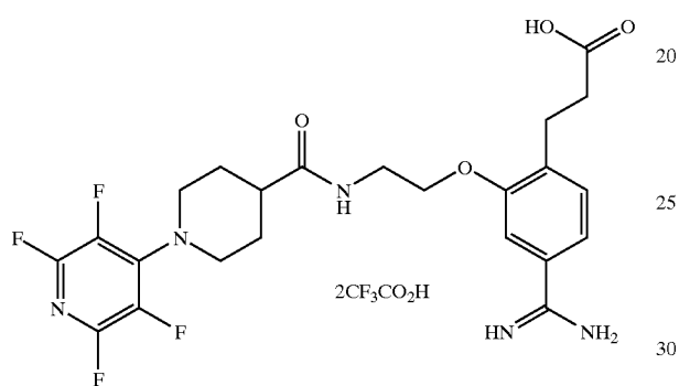
Compound of Example 17
