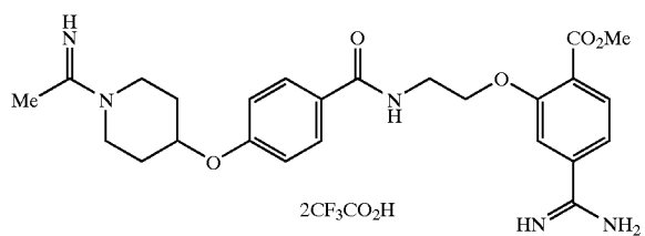
Compound of Example 38
