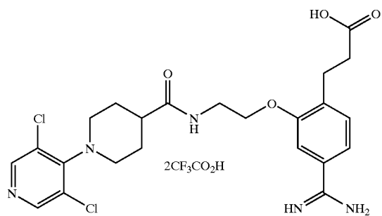
Compound of example 20
