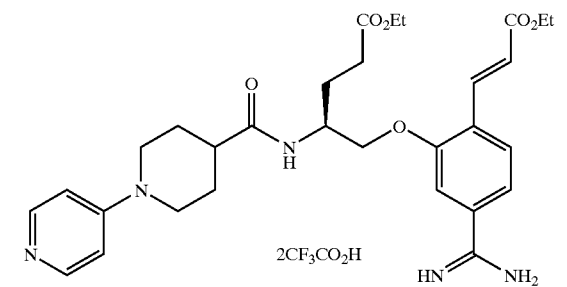
Compound of Example 32
