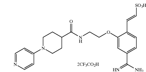
Compound of example 41
