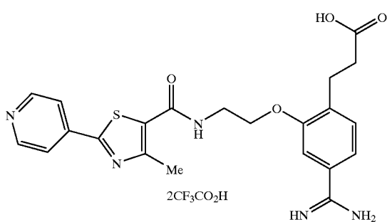
Compound of Example 21
