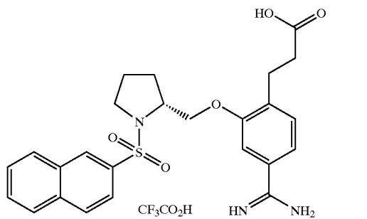
Compound of Example 27
