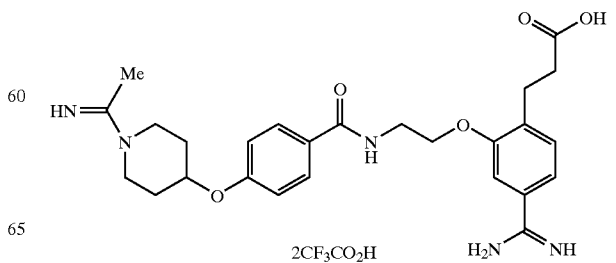
Compound of Example 4
