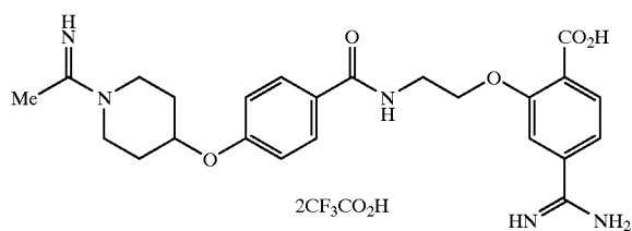
Compound of Example 40
