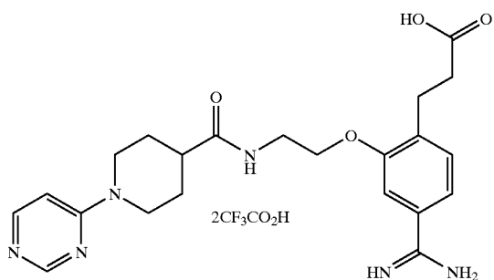
Compound of Example 25
