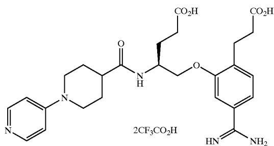
Compound of Example 34
