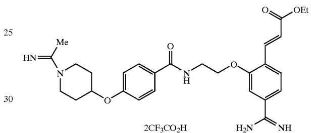
Compound of Example 2
