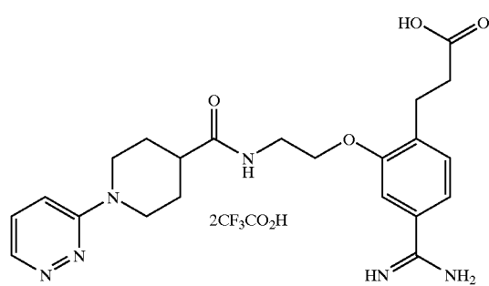
Compound of Example 23
