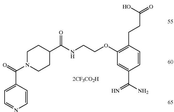
Compound of Example 19
