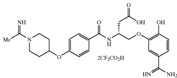
Compound of Example 29
