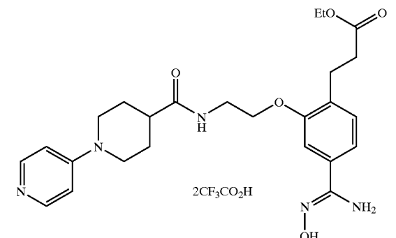
Compound of Example 31
