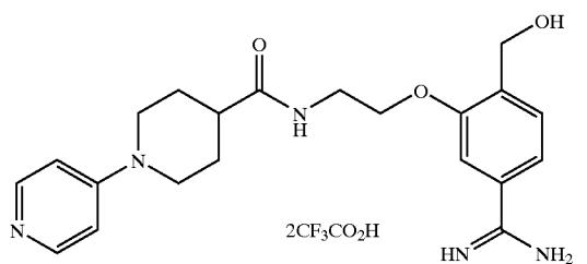
Compound of Example 38
