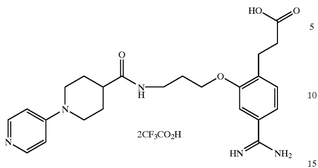
Compound of Example 16
