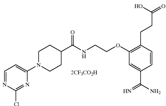
Compound of example 24
