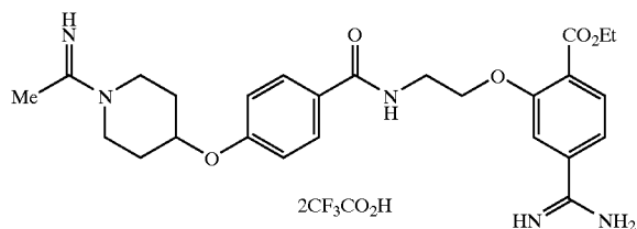
Compound of Example 39
