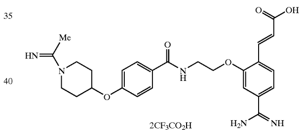
Compound of Example 3
