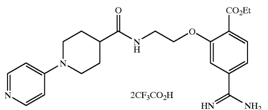
Compound of Example 35
