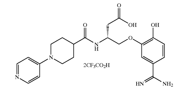
Compound of Example 29
