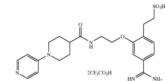
Compound of Example 42
