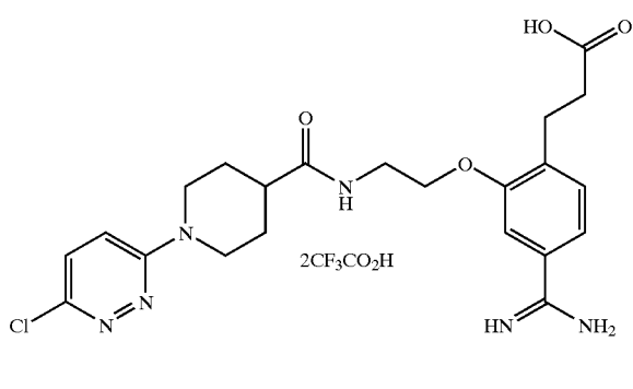
Compound of Example 22
