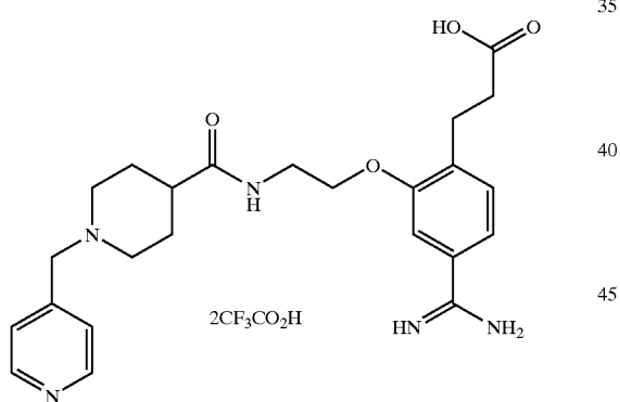
Compound of Example 18
