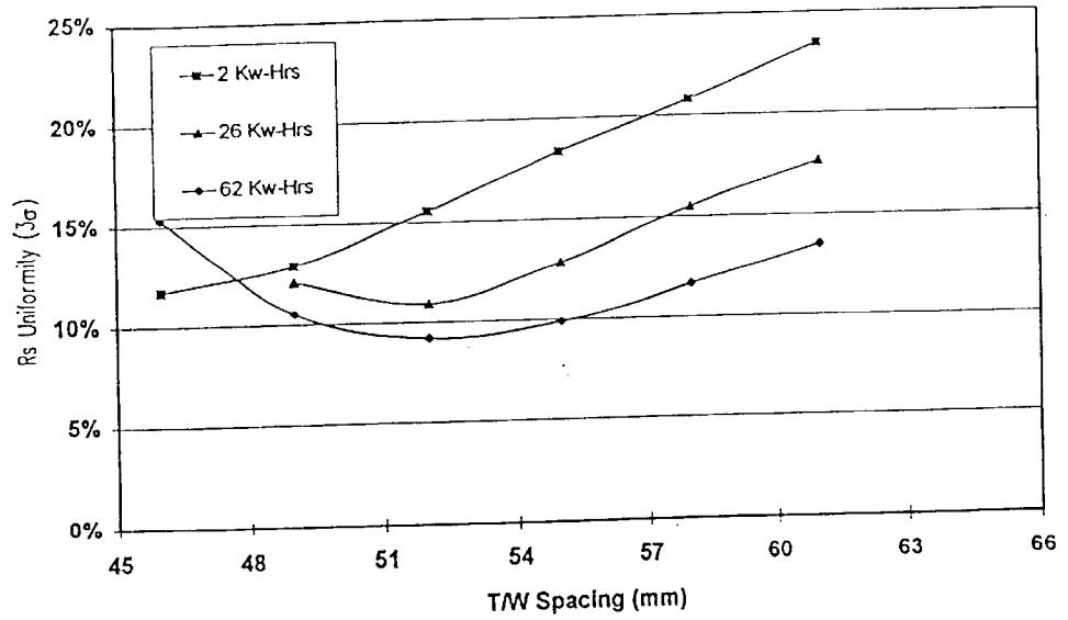
Uniformity vs. Target Life for Sample B
