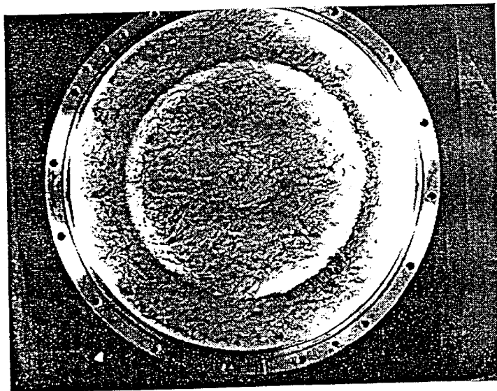
Sample B Target Surface Post Sputtering
