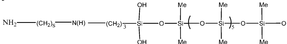
Compound I
