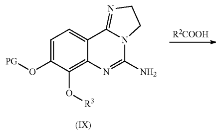
Reaction Scheme 4
