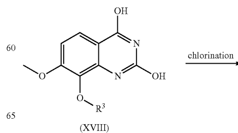
Reaction Scheme 5
