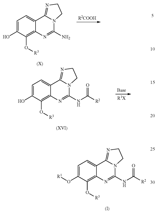
Reaction Scheme 3
