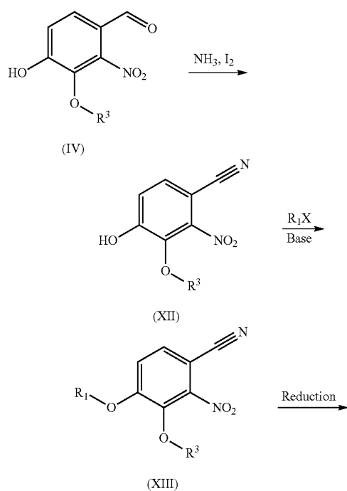
Reaction Scheme 2
