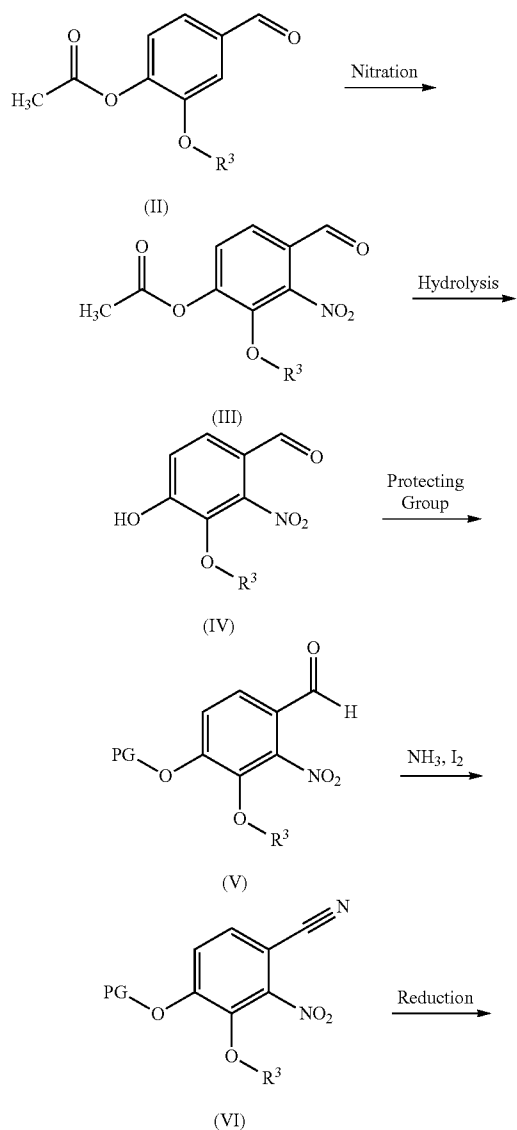
Reaction Scheme 1
