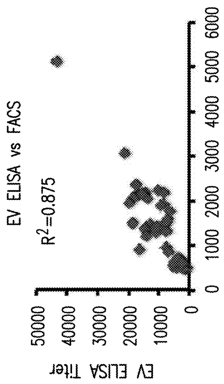
EV ELISA results correlate well with FACS
