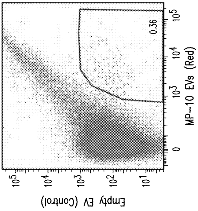
Staining profile of IgG + rabbit B cells
