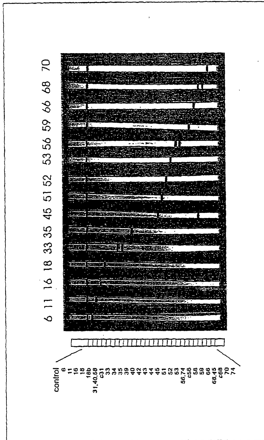
Figure 11: Typical HPV LiPA patterns
