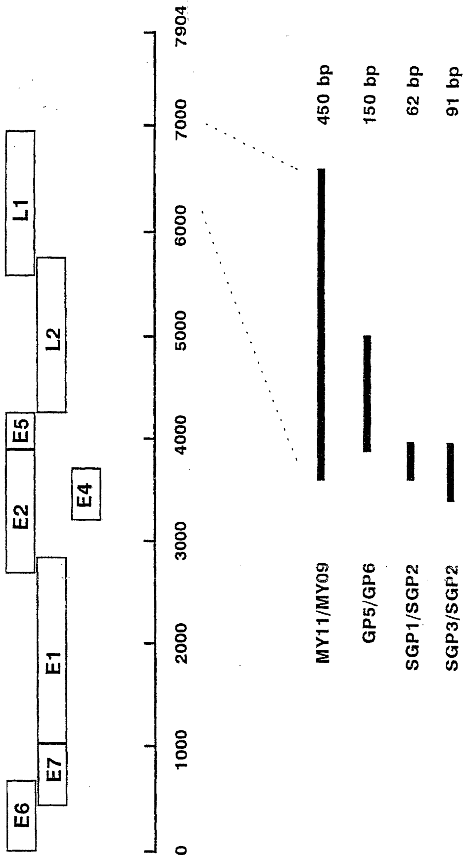
Figure 2: Outline of the HPV DNA genome
