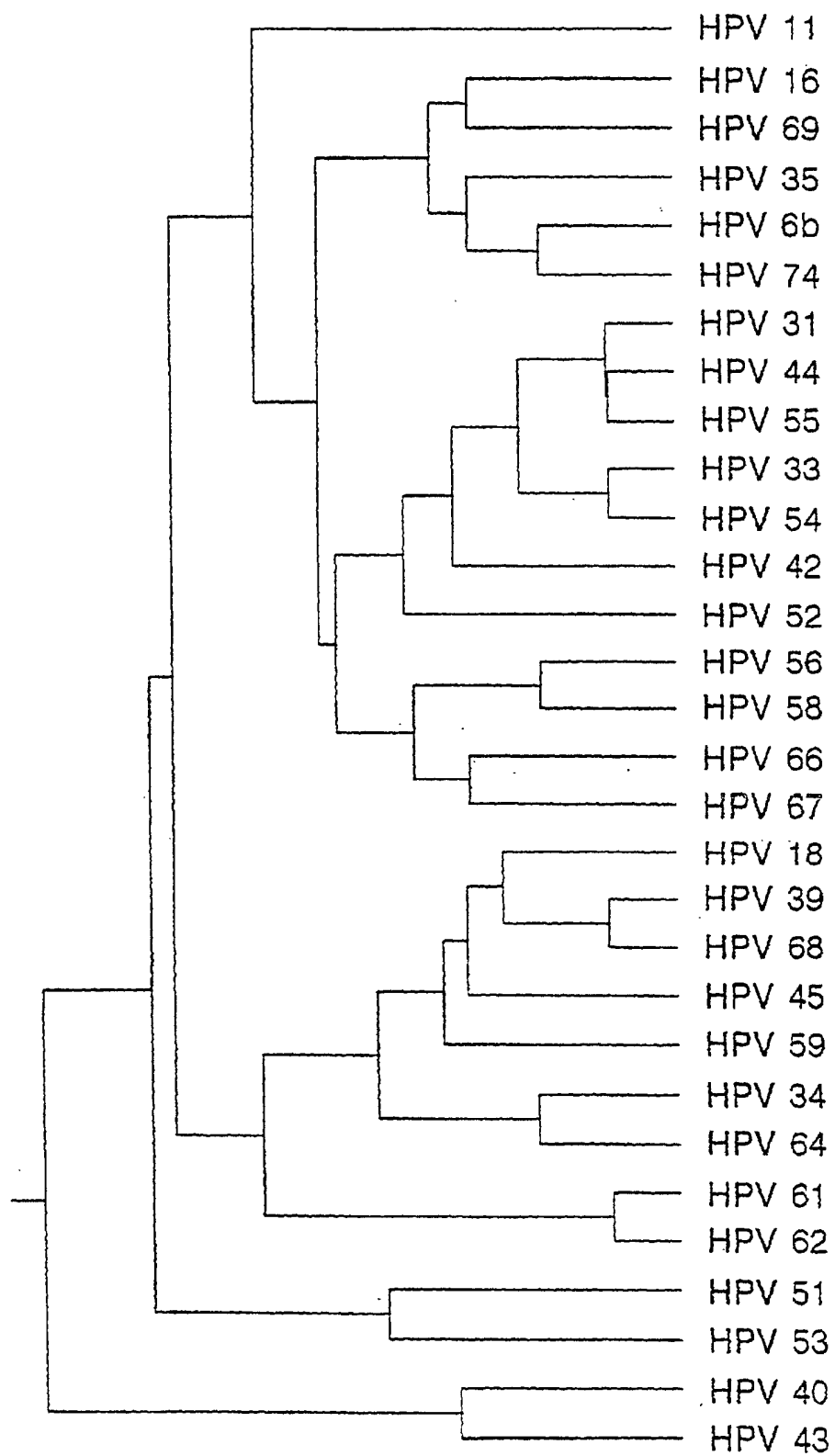
Figure 4: Phylogenetic tree of HPV sequences between the B and C regions
