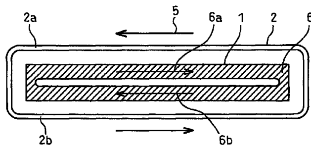
Fig.2 - PRIOR ART
