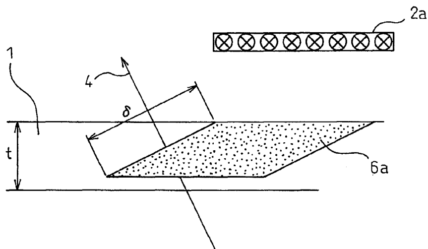
Fig.4 - PRIOR ART
