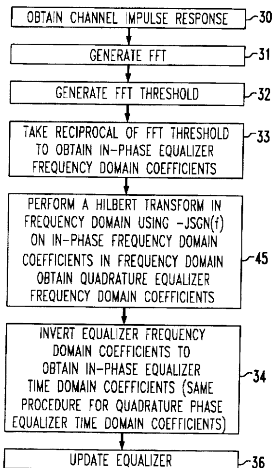
FIG. 16 CHANNEL SOUNDING PROCESS
