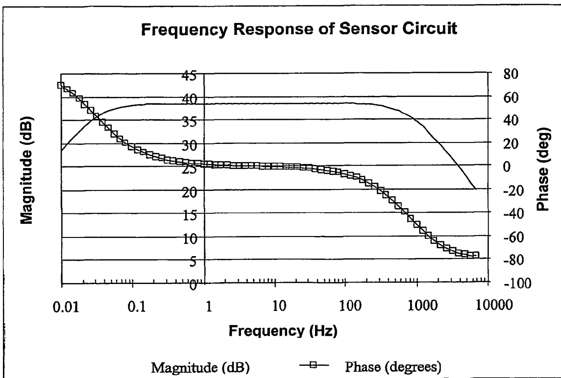
Figure 6: Frequency response of sensor
