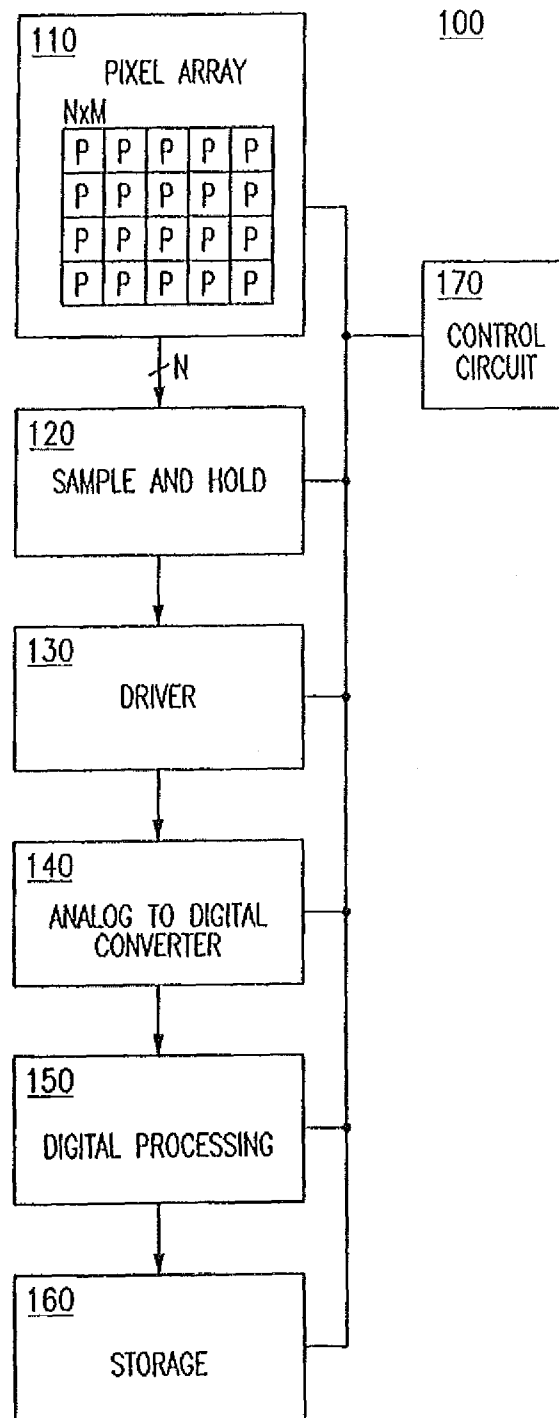
FIG. 1 (PRIOR ART)
