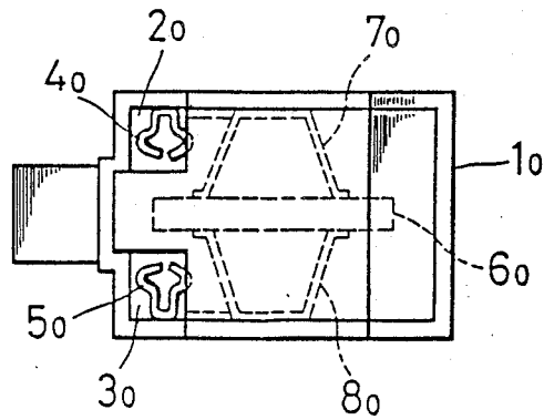
Fig. 5 PRIOR ART
