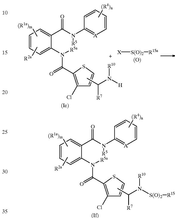
Reaction Scheme 5
