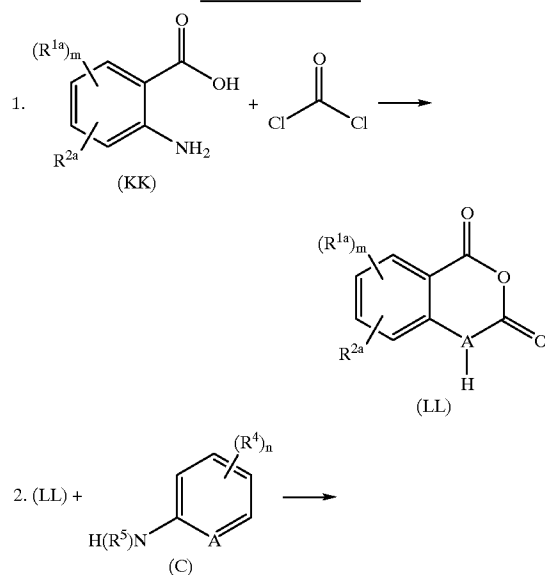
Reaction Scheme 20
