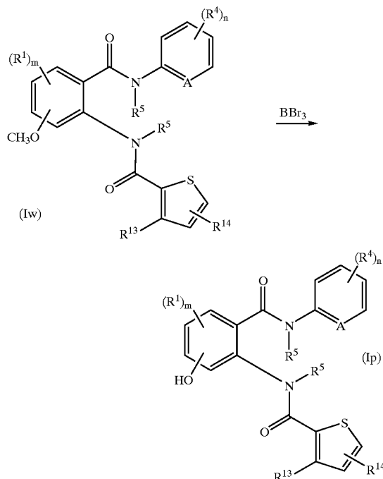
Reaction Scheme 17
