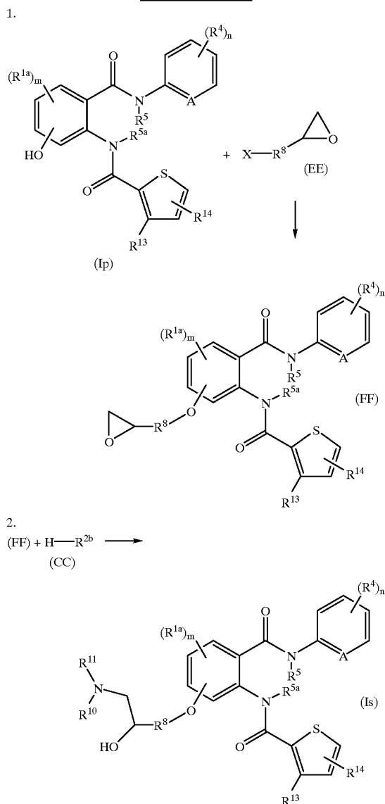
Reaction Scheme 14
