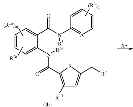
Reaction Scheme 3
