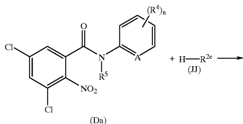
Reaction Scheme 19
