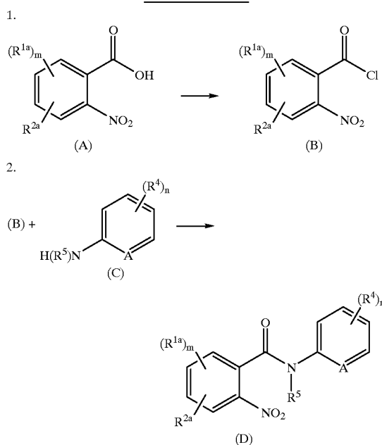
Reaction Scheme 1
