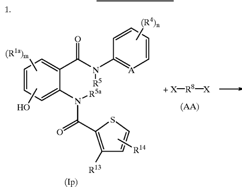
Reaction Scheme 12
