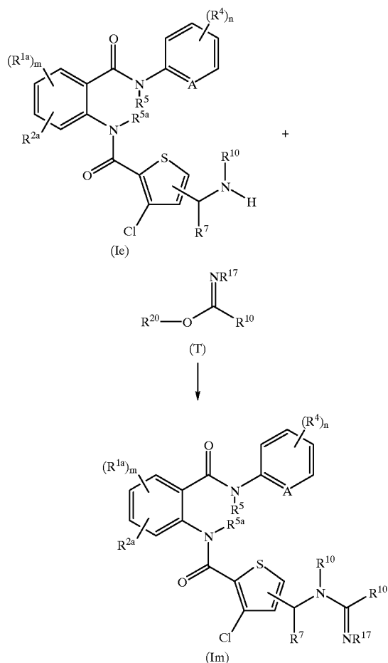
Reaction Scheme 9
