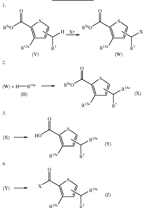
Reaction Scheme 11
