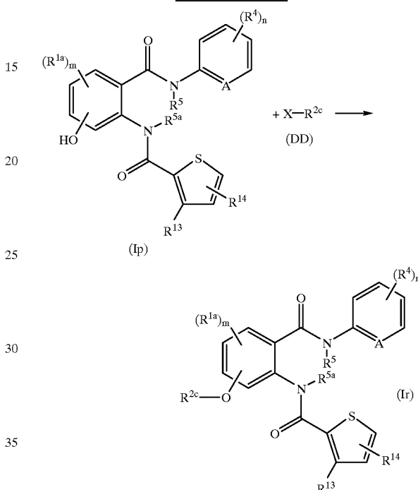
Reaction Scheme 13
