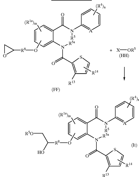
Reaction Scheme 15
