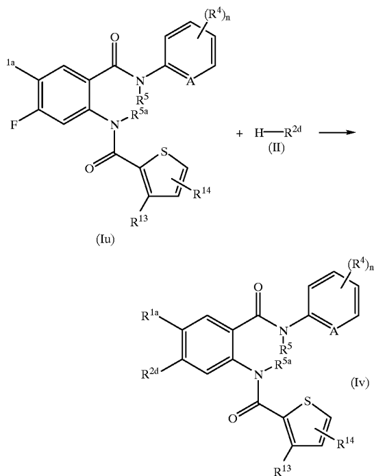
Reaction Scheme 16
