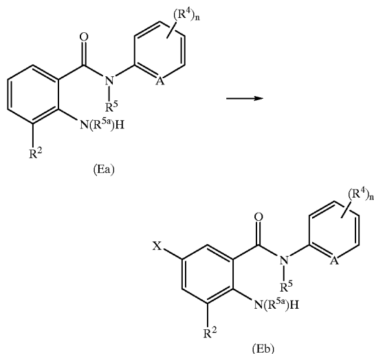
Reaction Scheme 18
