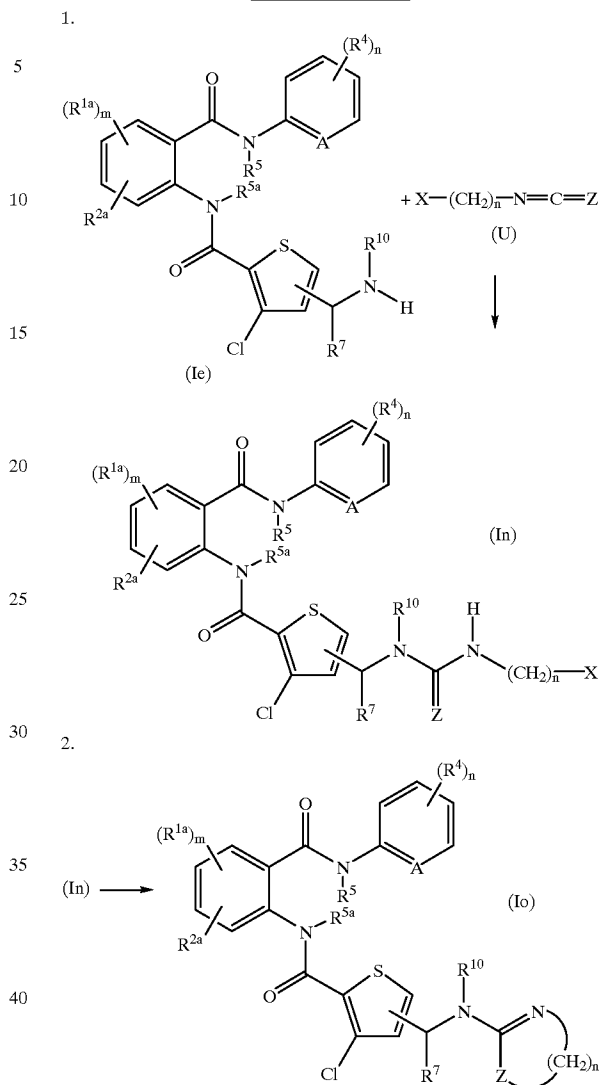
Reaction Scheme 10
