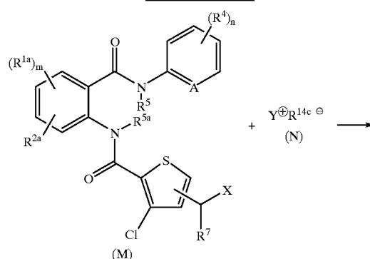
Reaction Scheme 4
