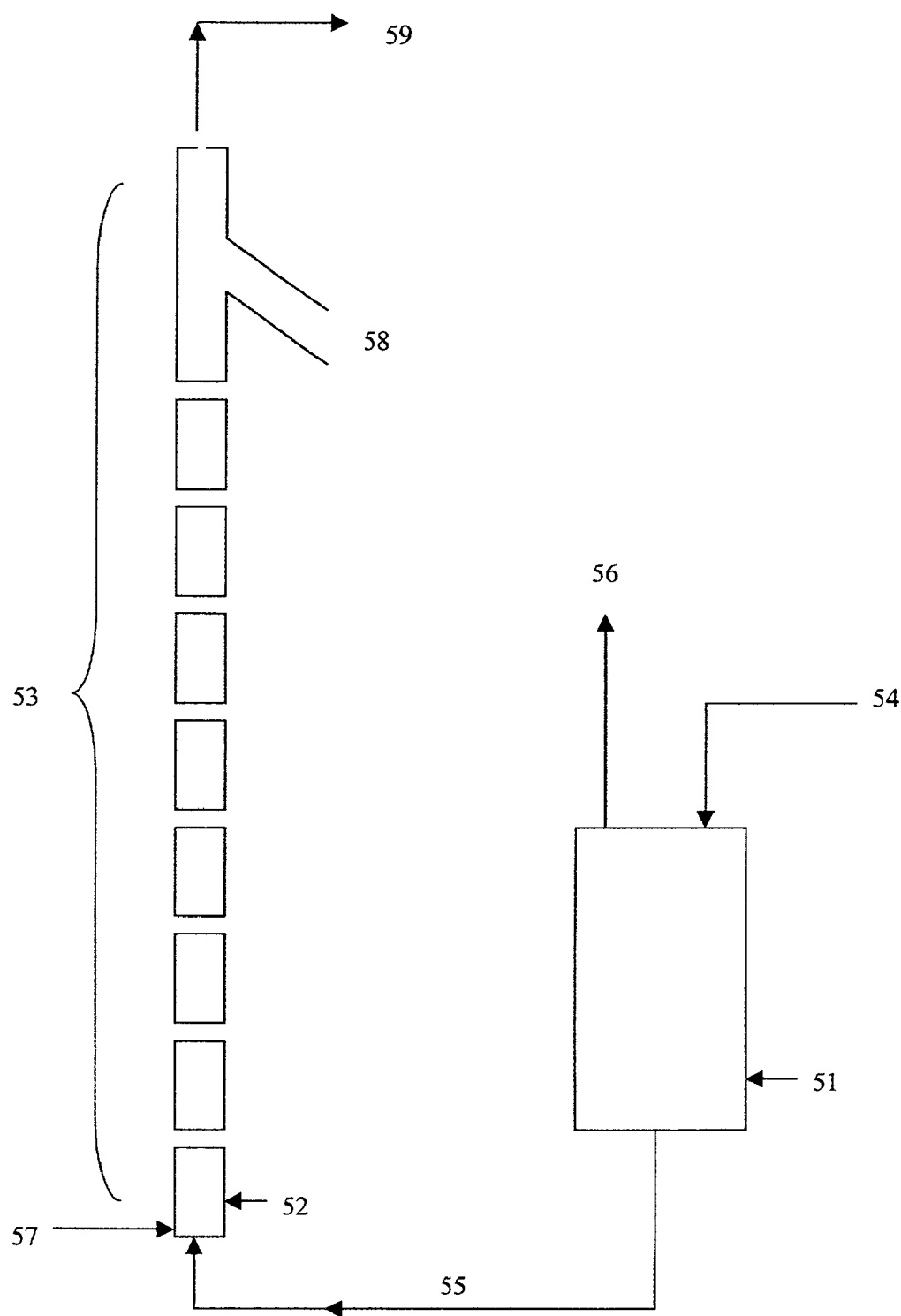
FIGURE 6 - OPERATION WITH PRE-REACTOR
