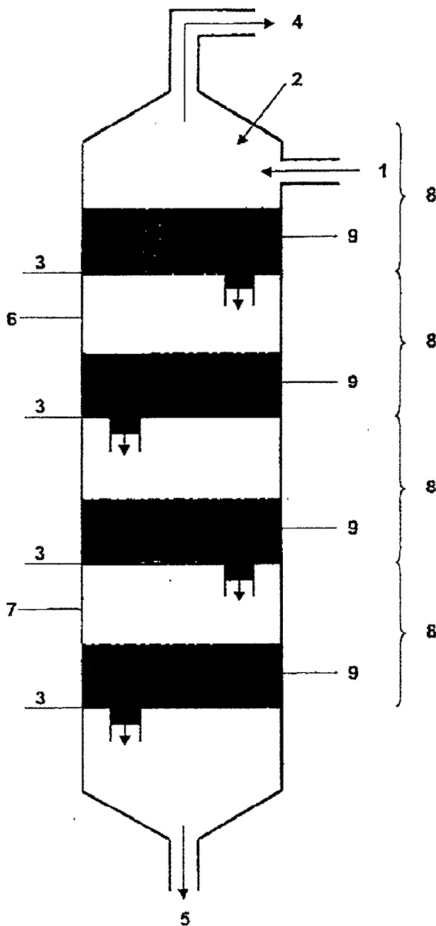
FIGURE 1. MULTI-STAGED COLUMN REACTOR
