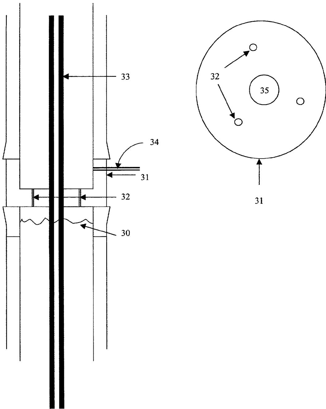
FIGURE 5A - INTERNAL COLUMN SECTION AND BARRIER
