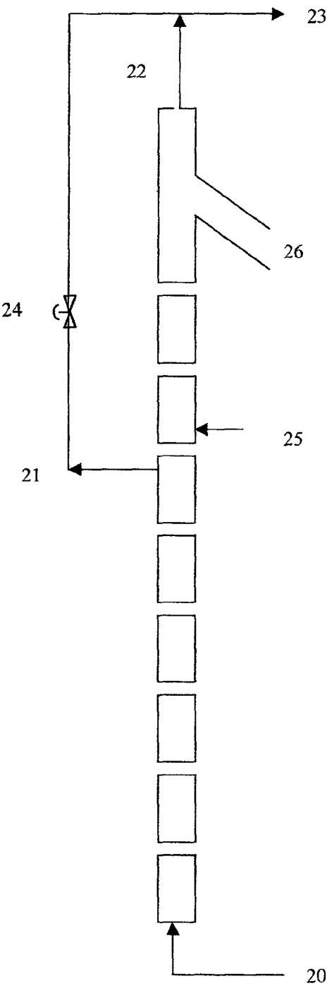
FIGURE 4 - MULTI-STAGED COLUMN REACTOR WITH CAPABILITY FOR WATER REMOVAL
