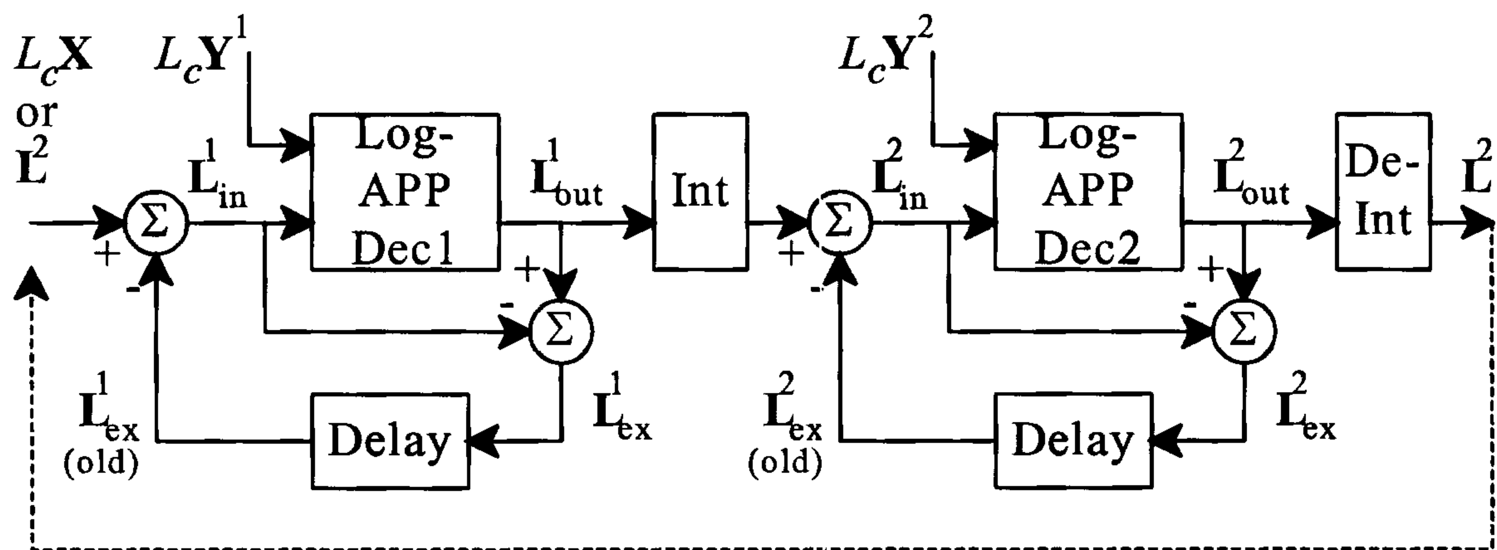
Fig. 3(Prior Art):
