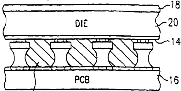
VIA IN SUBSTRATE (USUALLY THE SMALLEST JOINT CROSS-SECTION)
