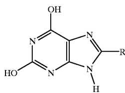
R=H=Xanthine
