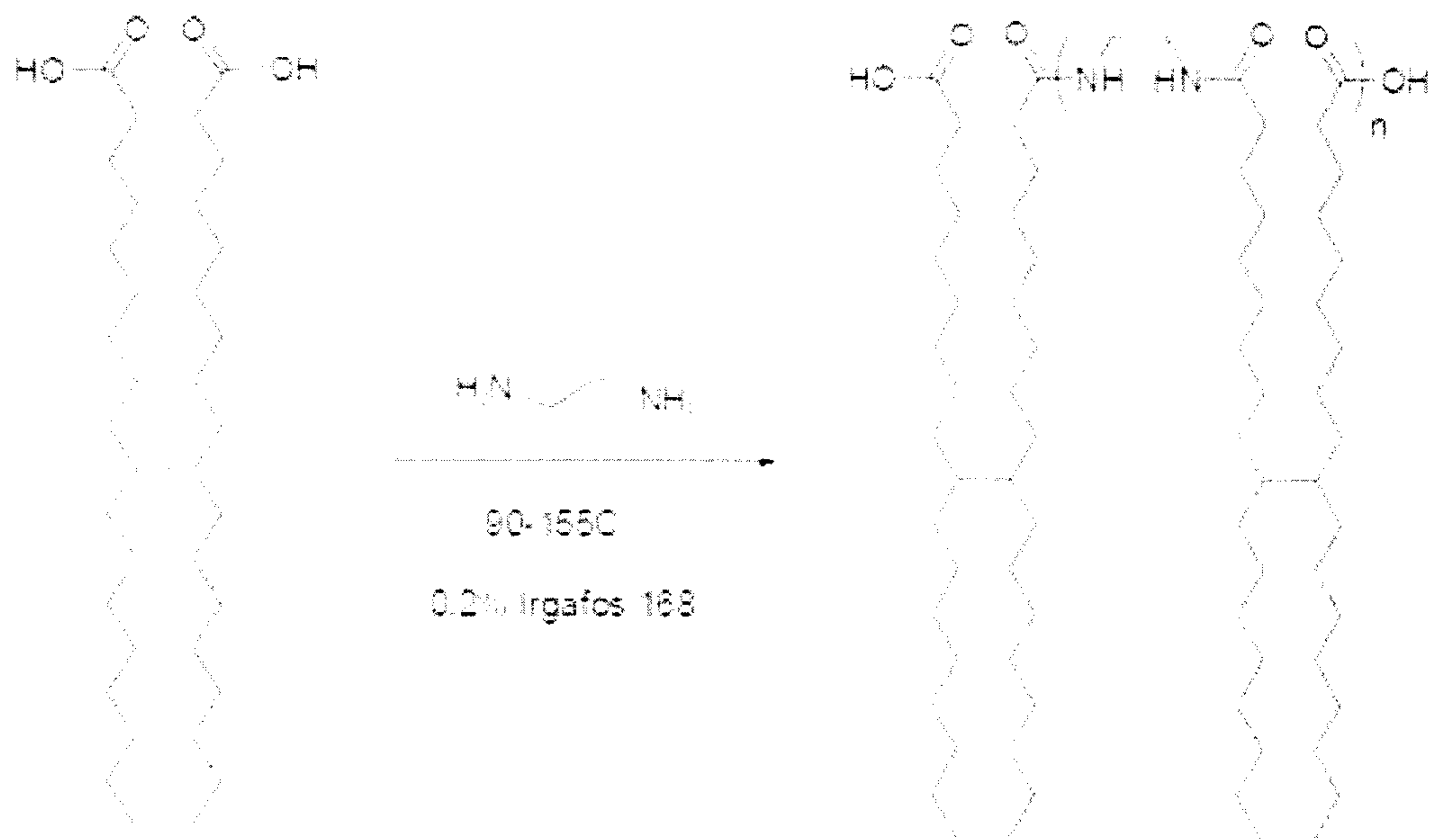
Scheme 1 Where n may be 0 to about 20, about 0 to about 15, or about 0 to about 10.
