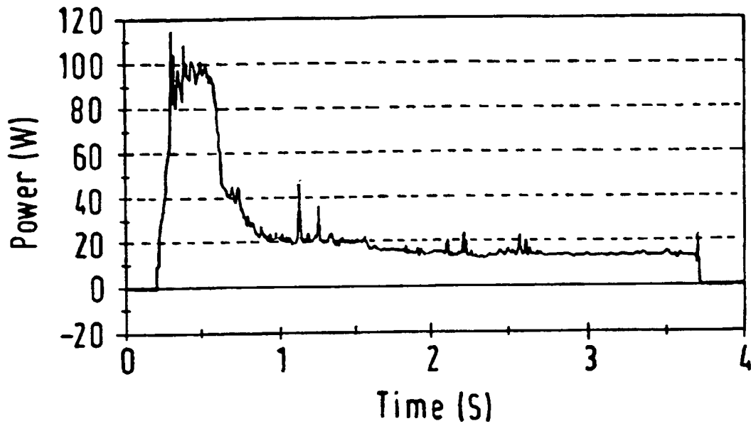
FIG. 2(a) POWER
