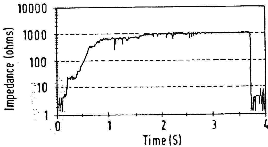
FIG. 2(b) IMPEDANCE
