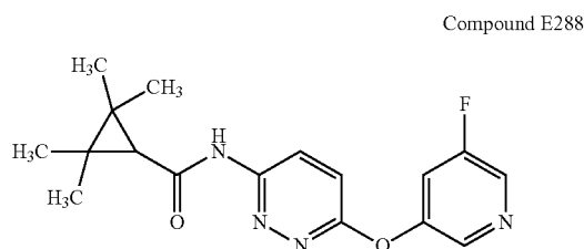
N-[6-[(5-fluoro-3-pyridyl)oxy]pyridazin-3-yl]-2,2,3,3-tetramethyl-cyclopropanecarboxamide
