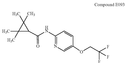
2,2,3,3-tetramethyl-N-[5-(2,2,2-trifluoroethoxy)-2-pyridyl]cyclopropanecarboxamide
