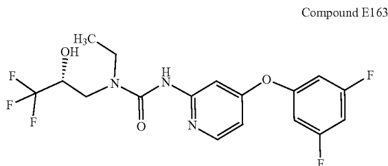
3-[4-(3,5-difluorophenoxy)-2-pyridyl]-1-ethyl-1-[(2R)-3,3,3-trifluoro-2-hydroxy-propyl]urea
