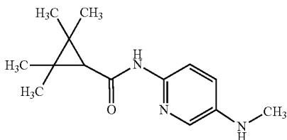
2,2,3,3-tetramethyl-N-[5-(methylamino)-2-pyridyl] cyclopropanecarboxamide
