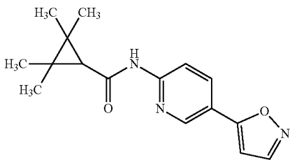
N-(5-isoxazol-5-yl-2-pyridyl)-2,2,3,3-tetramethylcyclopropanecarboxamide
