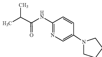
2-methyl-N-(5-pyrrolidin-1-yl-2-pyridyl)propanamide
