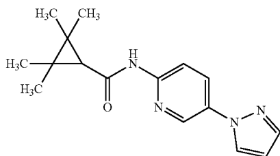
2,2,3,3-tetramethyl-N-(5-pyrazol-1-yl-2-pyridyl)cyclopropanecarboxamide
