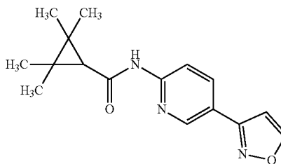
N-(5-isoxazol-3-yl-2-pyridyl)-2,2,3,3-tetramethylcyclopropanecarboxamide
