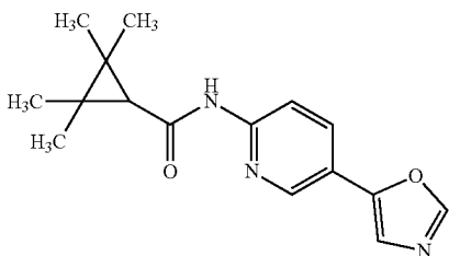
2,2,3,3-tetramethyl-N-(5-oxazol-5-yl-2-pyridyl)cyclopropanecarboxamide
