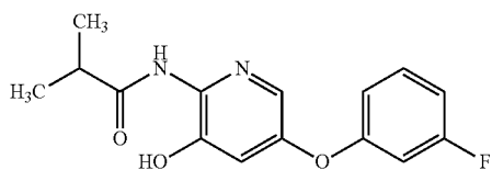
N-[5-(3-fluorophenoxy)-3-hydroxy-2-pyridyl]-2-methyl-propanamide
