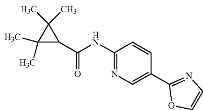
2,2,3,3-tetramethyl-N-(5-oxazol-2-yl-2-pyridyl)cyclopropanecarboxamide
