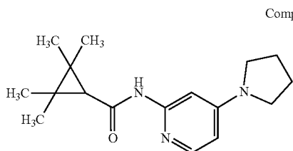
2,2,3,3-tetramethyl-N-(4-pyrrolidin-1-yl-2-pyridyl) cyclopropanecarboxamide
