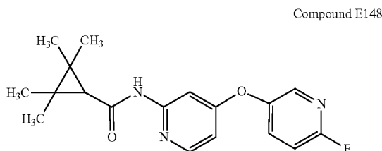
N-[4-[(6-fluoro-3-pyridyl)oxy]-2-pyridyl]-2,2,3,3-tetramethylcyclopropanecarboxamide
