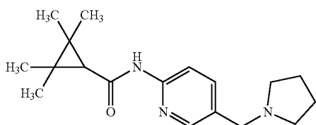
2,2,3,3-tetramethyl-N-[5-(pyrrolidin-1-ylmethyl)-2-pyridyl]cyclopropanecarboxamide
