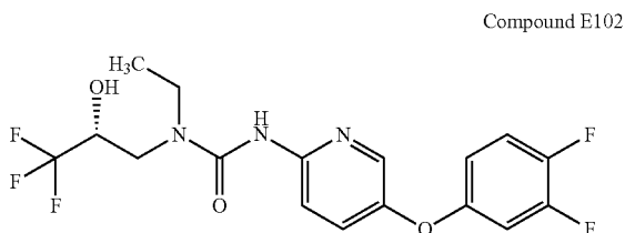
3-[5-(3,4-difluorophenoxy)-2-pyridyl]-1-ethyl-1- [(2R)-3,3,3-trifluoro-2-hydroxy-propyl]urea
