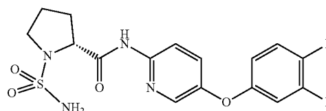
Compound E277
