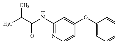
2-methyl-N-(4-phenoxy-2-pyridyl)propanamide
