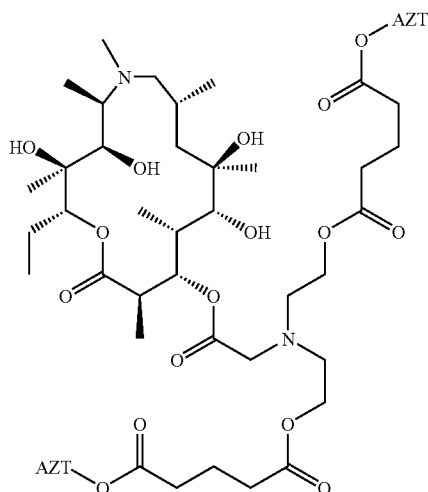
Compound 101
