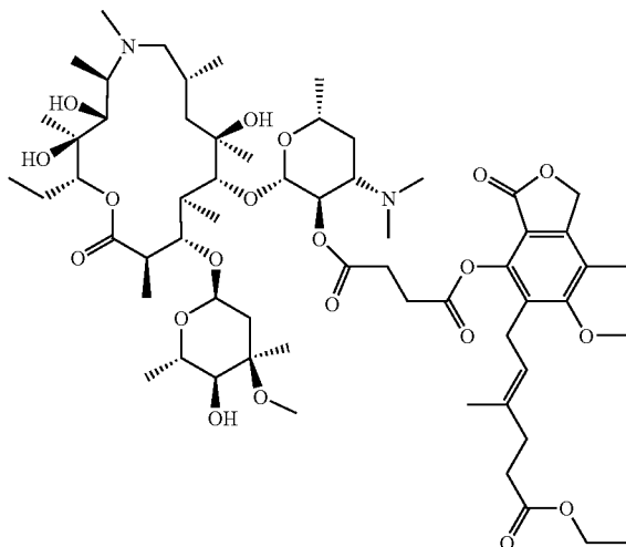
Compound 69
