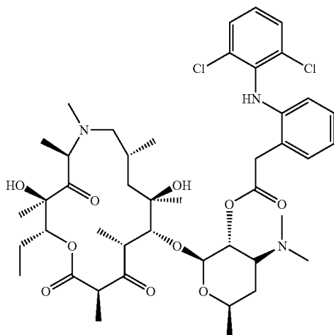
Compound 54
