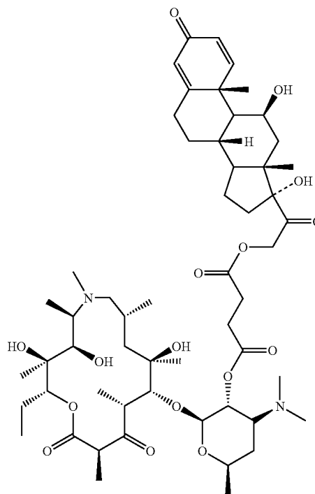
Compound 86
