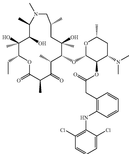
Compound 53
