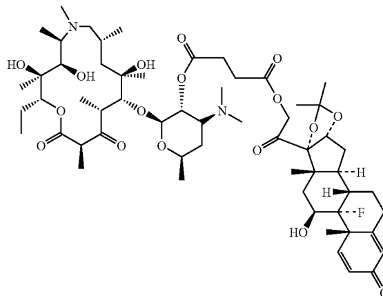
Compound 85
