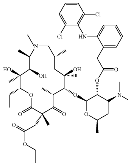
Compound 55
