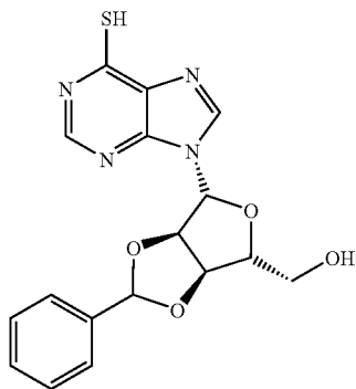
Compound 92
