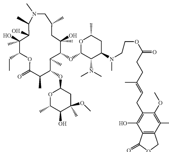
Compound 73
