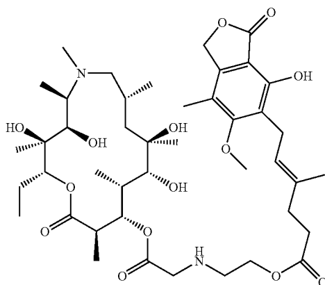
Compound 71
