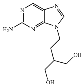
Pencyclovir
