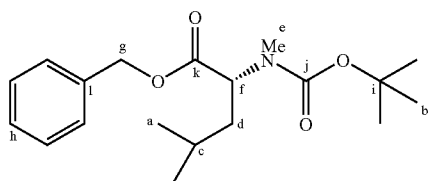
N-Boc N-Methyl benzyl D-leucinate (Compound 47 )
