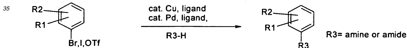
Scheme 9:
