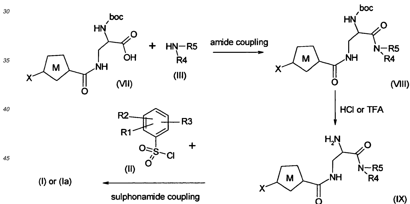
Scheme 2:
