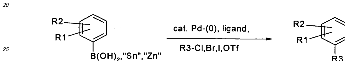
Scheme 8:
