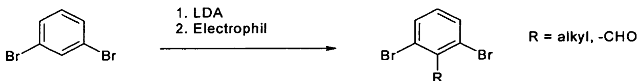
Scheme 6:
