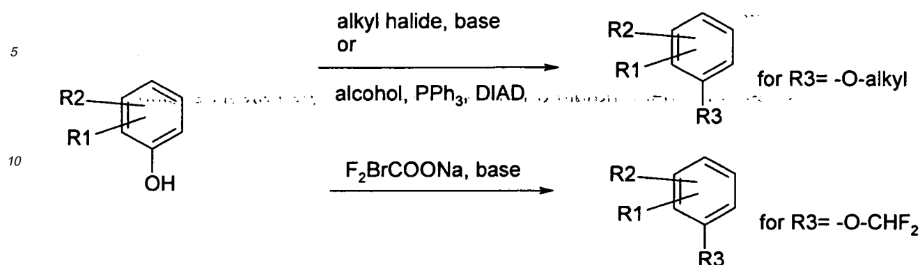
Scheme 10:
