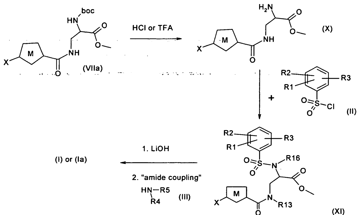
Scheme 3:
