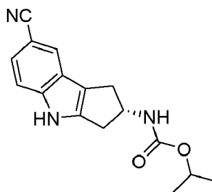
(Formula III);
