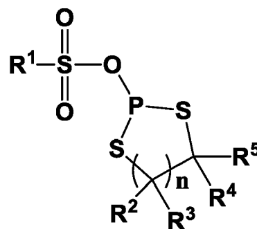
[Chemical Formula 1-3]
