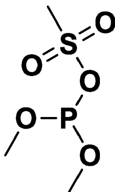
[Compound B]
