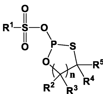
[Chemical Formula 1-2]
