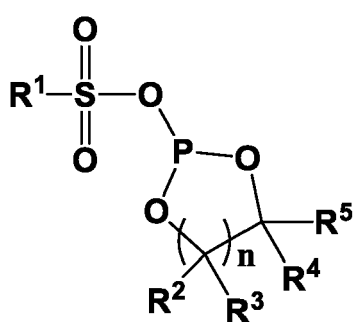
[Chemical Formula 1-1]
