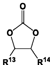
[Chemical Formula 4]
