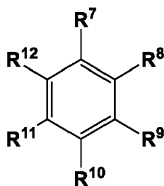
[Chemical Formula 3]
