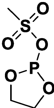
[Compound A]
