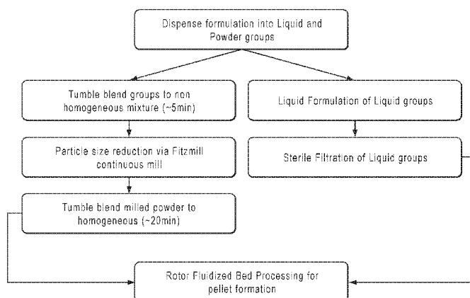
FIG. 8: Pelletizing Process
