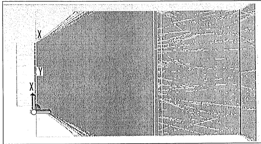
TOTAL-IRRADANCE MAP FOR EXITING FLUX NORMALIZED TO AVERAGE EMITED RADIANCE (GND AND SURFACE SOURCES) EXIT BLOCK BACK SURFACE
