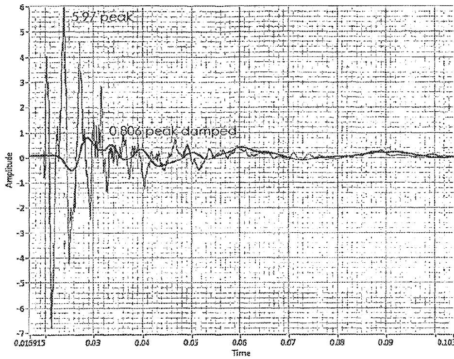
Test waveforms HiFi Platform
