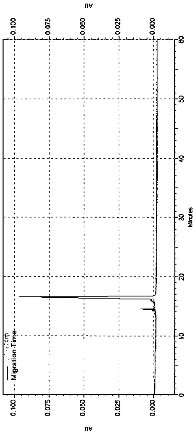
Fig.15 21-mer RNA synthesized by reverse direction (5'→3'), followed by HEG (Hexa-ethyloxyglycol) attachment
