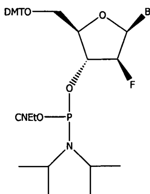
Structure (2)
