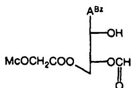
Structure 11.
