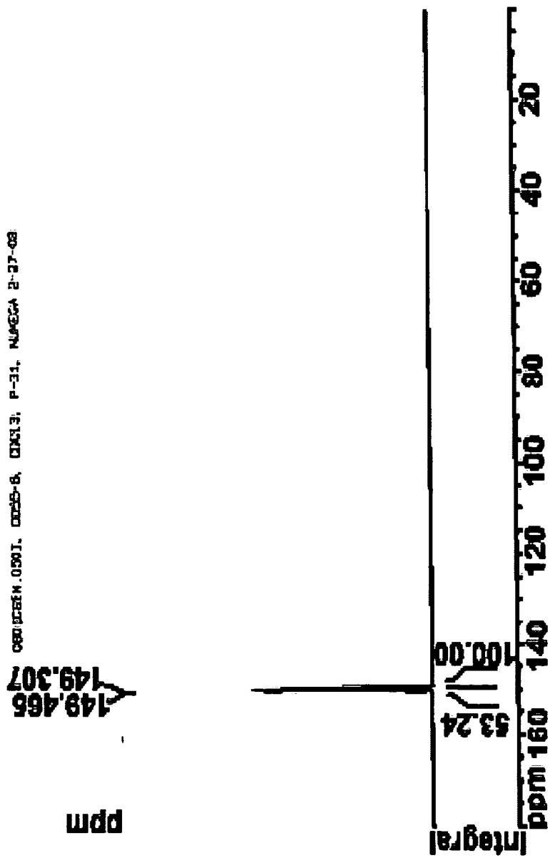
Fig.2. 31 P NMR spectrum of the compound (16a)
