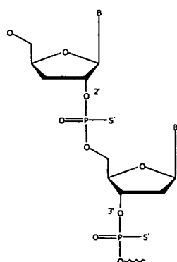
Structure (5). ( 2'-5'- linked DNA unit)
