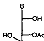
Structure 12
