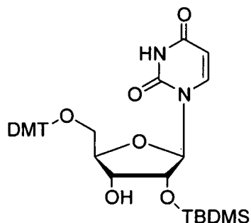
Structure (30)
