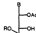
Structure 13
