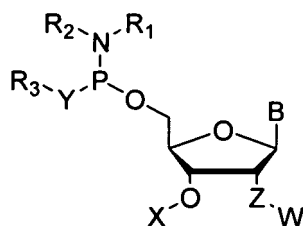
Structure (14)
