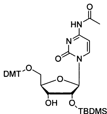
Structure (29)
