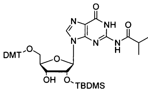
Structure (28)
