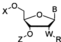
Structure (15)
