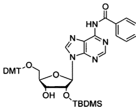
Structure (31).
