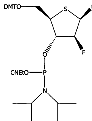
Structure (3)
