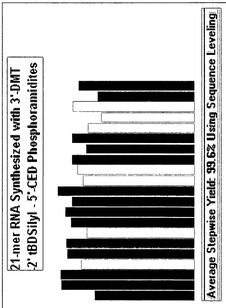
Fig. 8. Coupling Efficiency Trityl Histogram Notes (21 mer RNA Synthesis)
