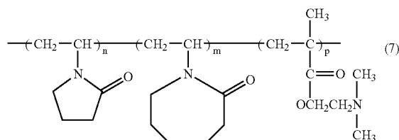
[Chemical formula 8]
