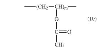
[Chemical formula 5]
