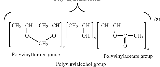
[Chemical formula 9]
