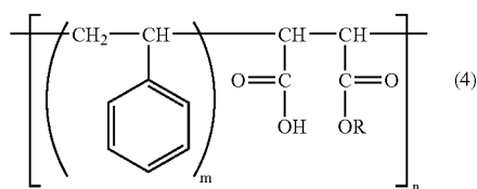
[Chemical formula 5]
