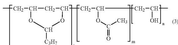
[Chemical formula 4]
