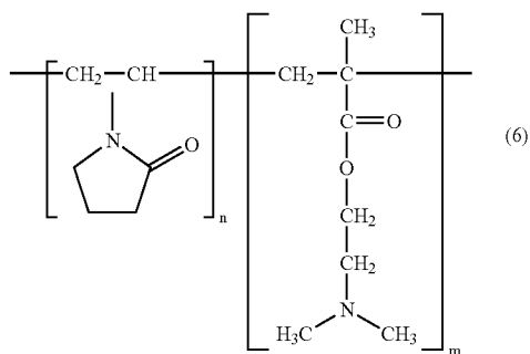
[Chemical formula 6]
