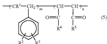
[Chemical formula 5]
