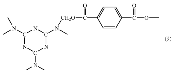
[Chemical formula 10]
