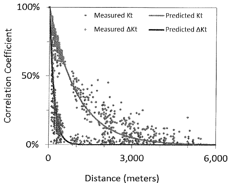
Fig. 13B. Correlation vs. Distance ( \Delta t=10 )
