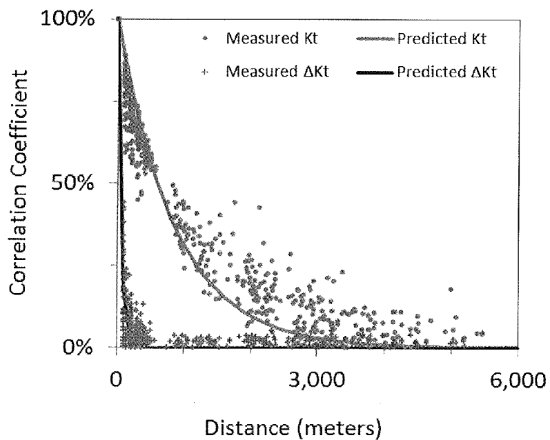
Fig. 13B. Correlation vs. Distance ( \Delta t=10 )
