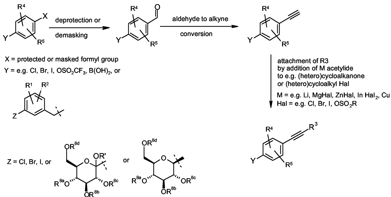
Scheme 6: Introduction of the Alkyne Moiety from an Aldehyde
