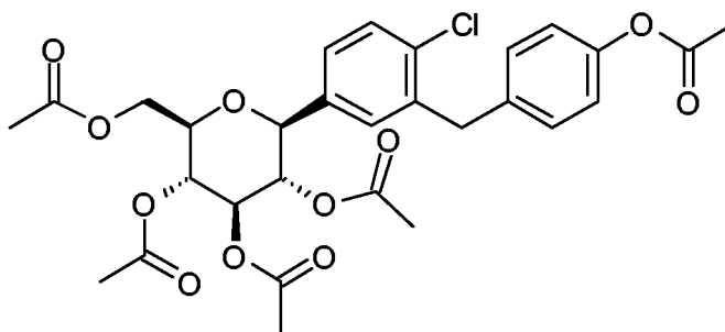
1-Chloro-2-(4-acetoxy-benzyl)-4-(2,3,4,6-tetra-O-acetyl- \beta -D-glucopyranos-1-yl)-benzene
