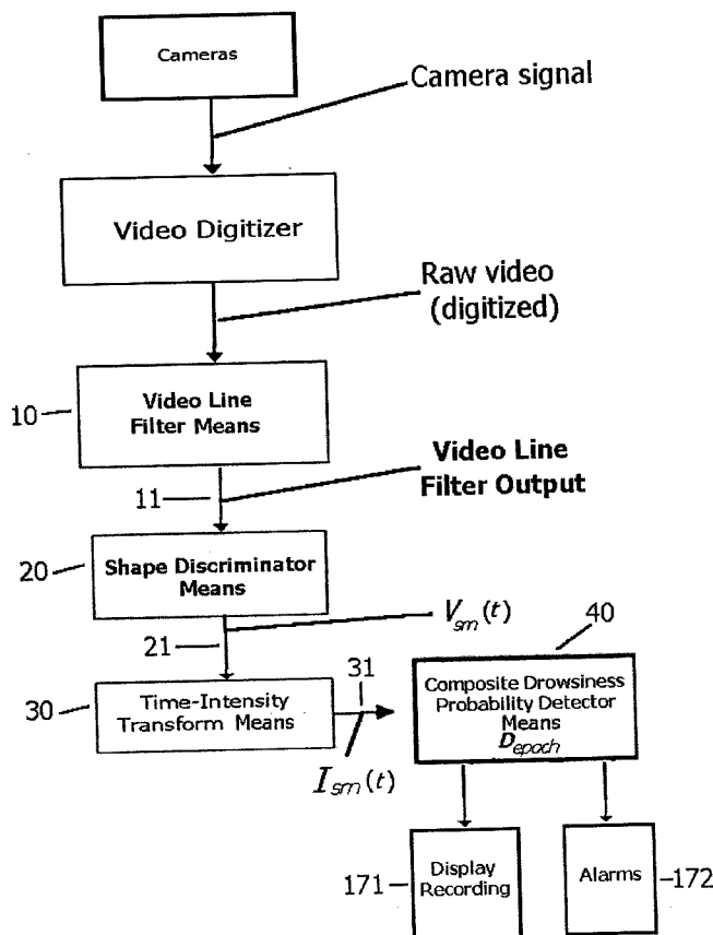
Signal Flow
