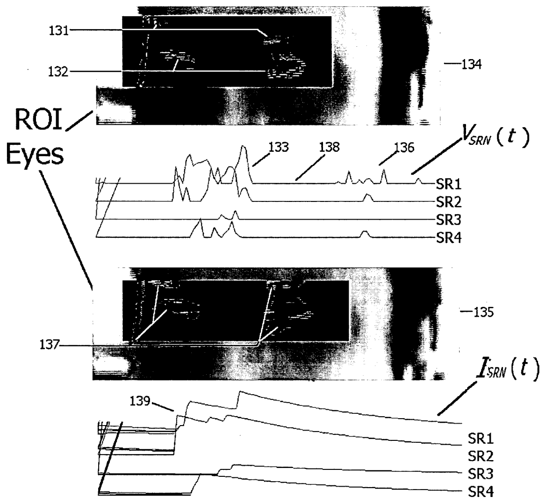
FIG. 9. SDM and TITM Outputs for Eye ROI
