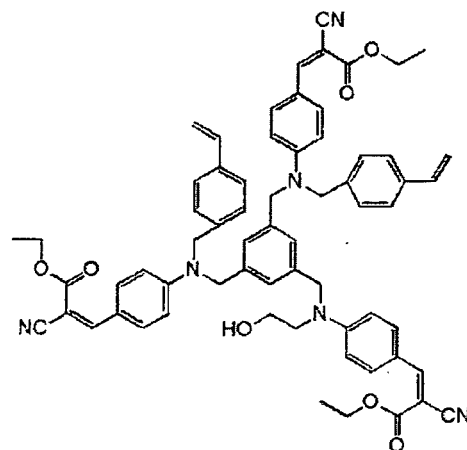
Compound No. 87
