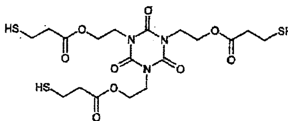
Compound No.125
