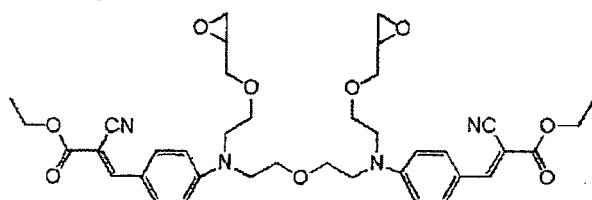
Compound No. 89
