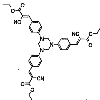
Compound No.23
