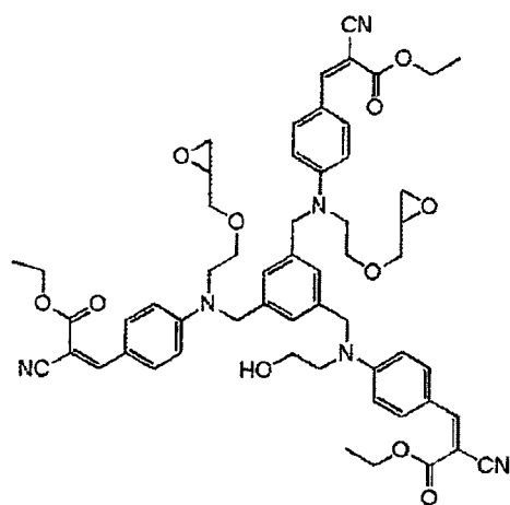
Compound No. 87
