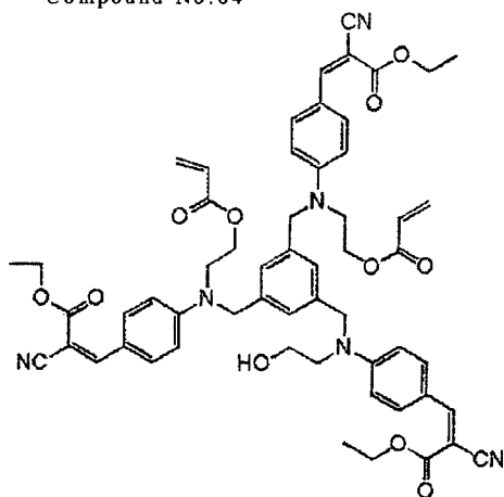
Compound No. 86
