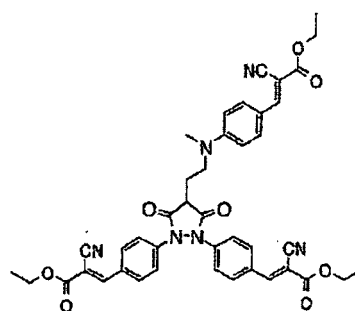
Compound No.42
