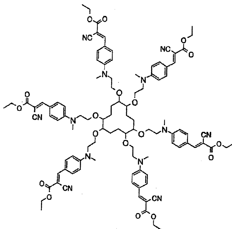
Compound No.28
