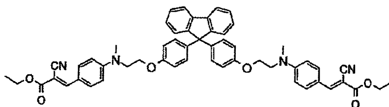
Compound No.38
