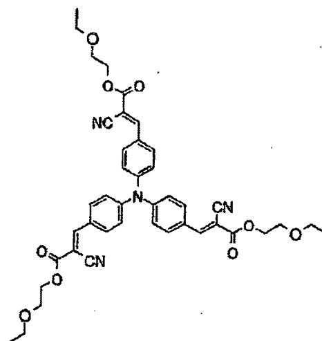
Compound No.6
