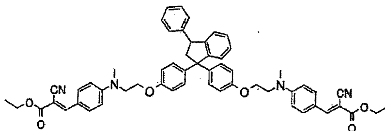
Compound No.40
