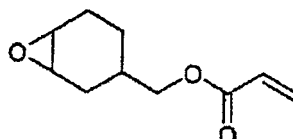
Compound No.124
