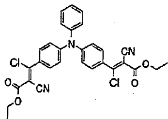
Compound No.16
