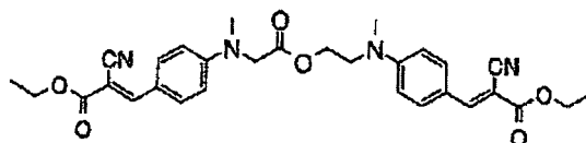
Compound No.34
