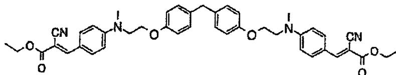
Compound No.38
