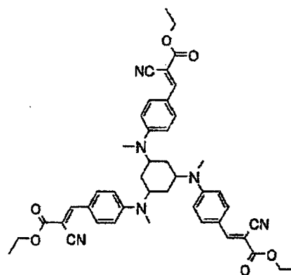
Compound No.24
