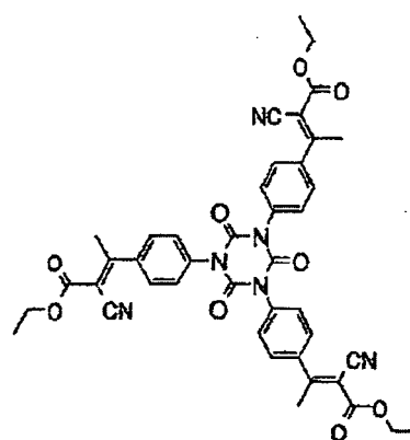
Compound No.22
