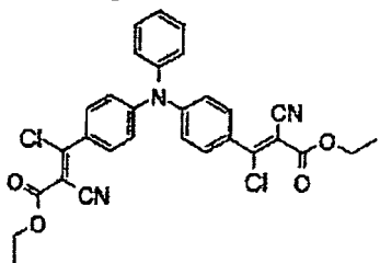
Compound No.18
