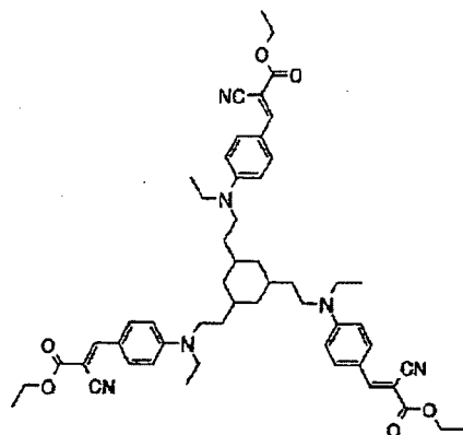
Compound No.43
