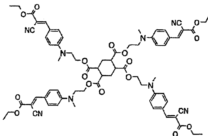
Compound No.26
