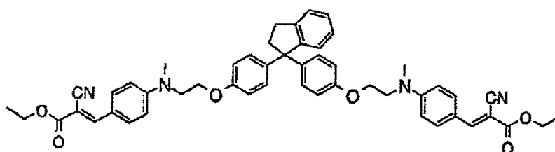
Compound No.40
