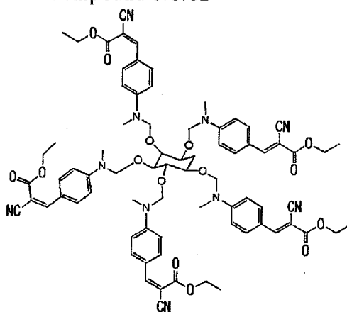
Compound No.82
