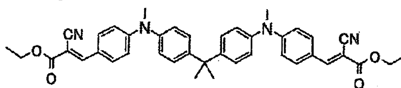
Compound No.13
