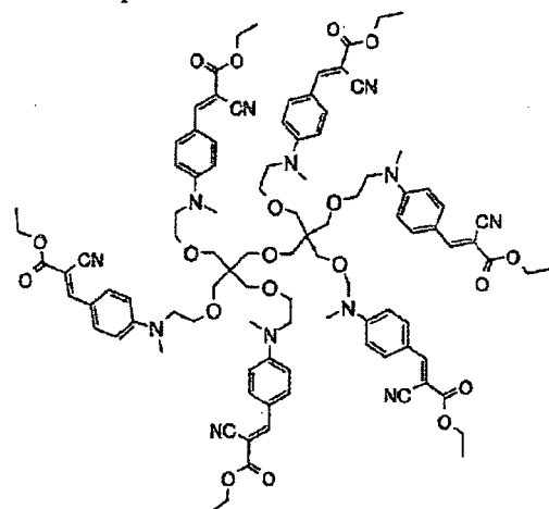
Compound No.45
