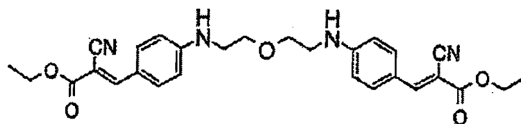
Compound No.10
