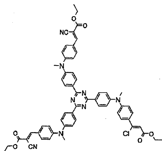
Compound No.23
