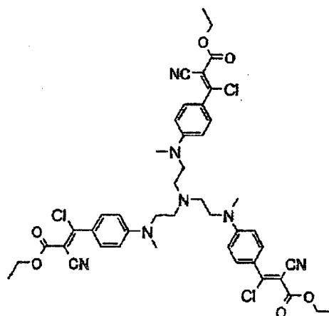
Compound No.19
