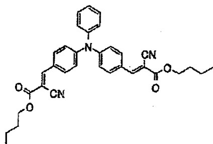
Compound No.3
