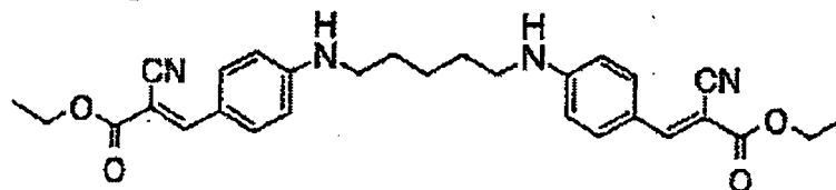
Compound No.13
