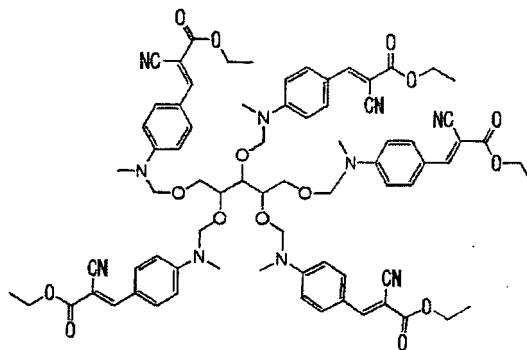
Compound No.82
