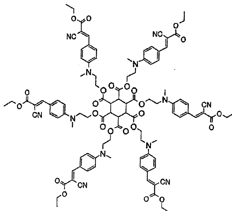
Compound No.28
