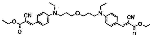
Compound No.32
