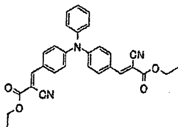
Compound No.1
