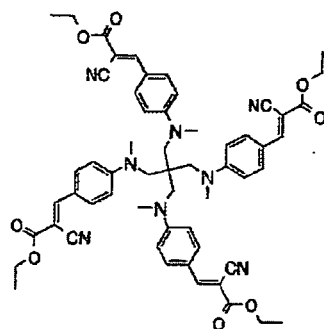
Compound No.45
