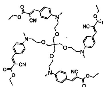
Compound No.44
