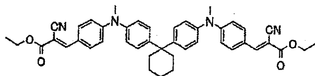
Compound No.37
