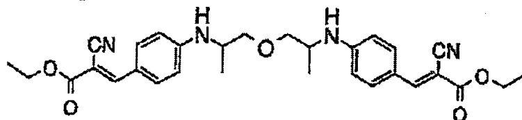
Compound No.11
