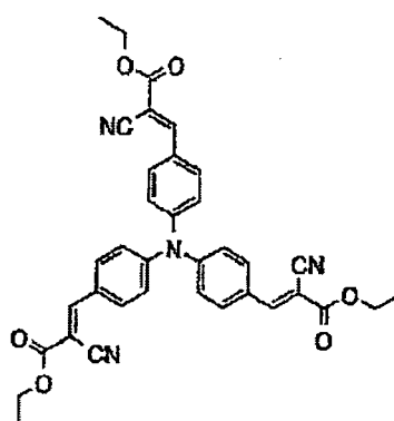
Compound No.4
