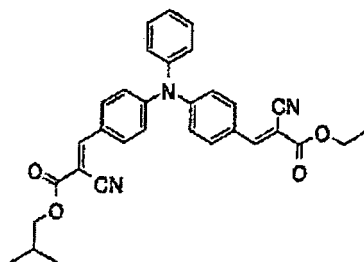
Compound No.29
