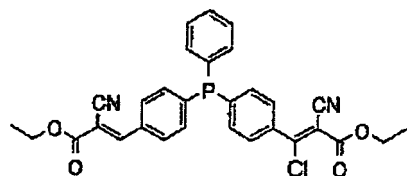
Compound No.16
