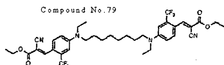
Compound No. 79
