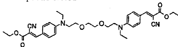
Compound No.33
