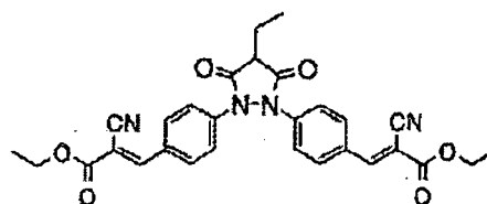
Compound No.8
