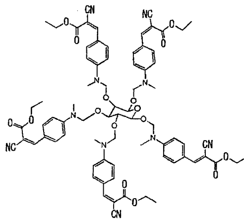
Compound No.83
