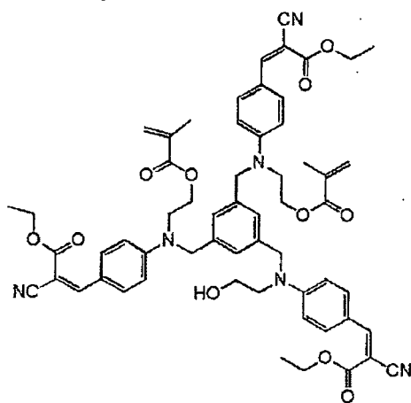
Compound No. 88
