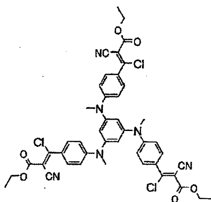
Compound No.20
