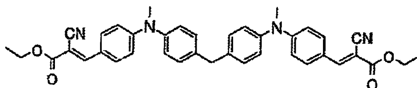
Compound No.12
