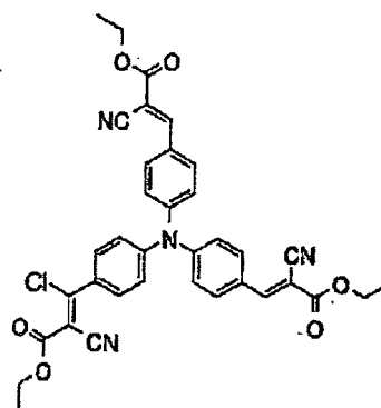
Compound No.30
