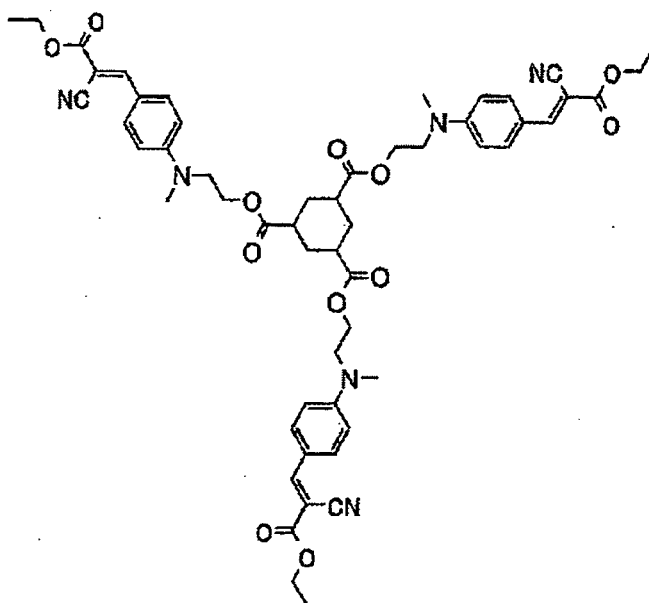
Compound No.26
