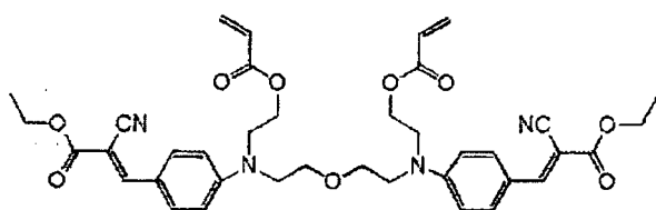
Compound No. 88
