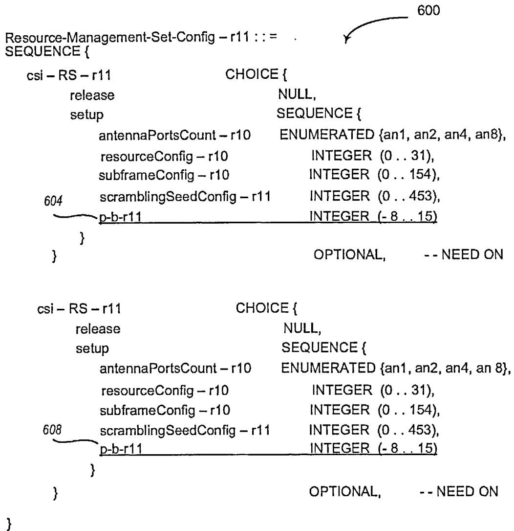
CoMP resource management set configuration signaling
