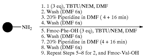
Scheme 1: Synthesis of Library 1
