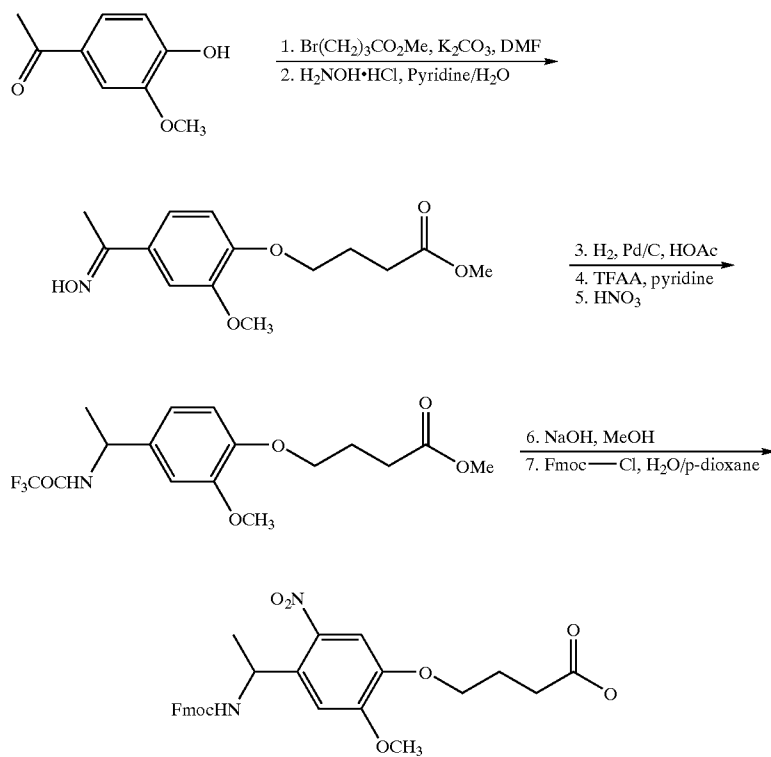
Scheme 4: Synthesis of 1
