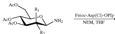
Scheme 10: Synthesis of 34 and 35
