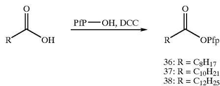
Scheme 11: Synthesis 36-38
