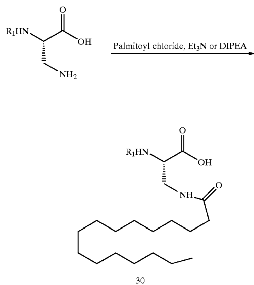
Scheme 7: Synthesis of 30
