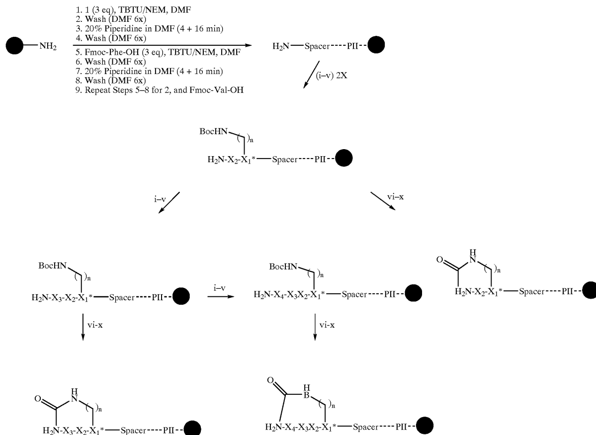
Scheme 12: Synthesis of Library 4, Variation A
