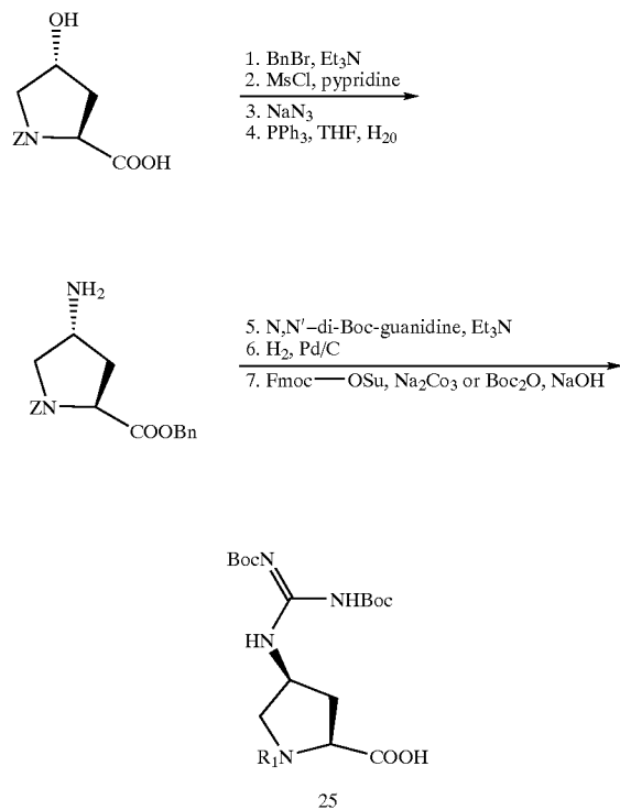
Scheme 6: Synthesis of 25
