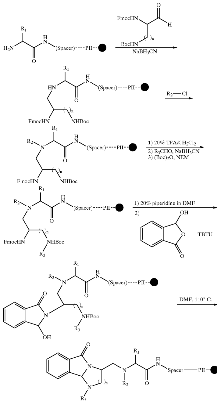
Scheme 13: Synthesis of Library 5
