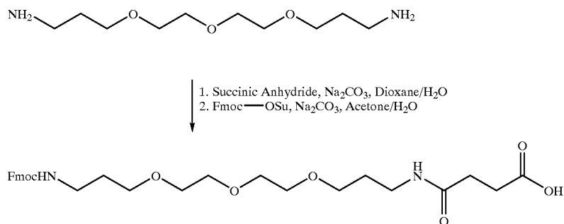
Scheme 5: Synthesis of 2
