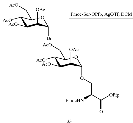
Scheme 9: Synthesis of 33
