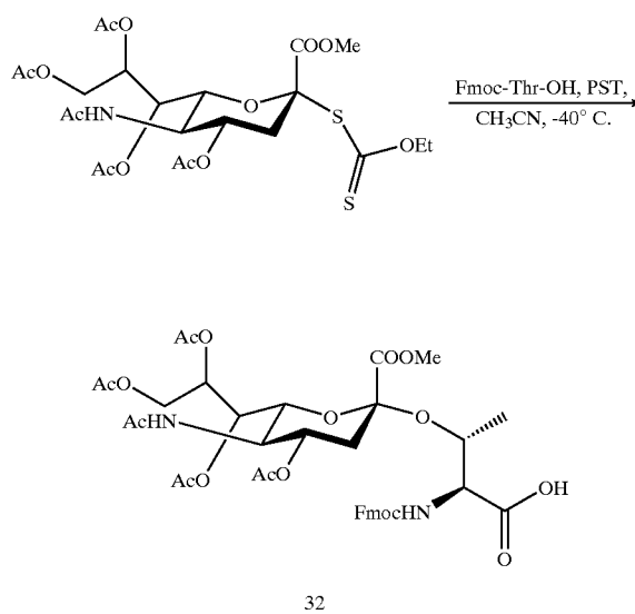
Scheme 8: Synthesis of 32
