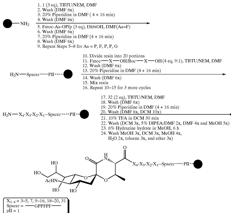
Scheme 2: Synthesis of Library 2
