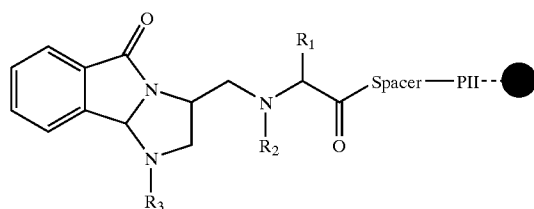
Synthesis of Library 5: Diazepine-like compounds
