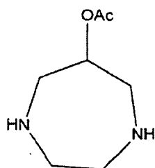
Compound 10
