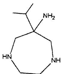
Compound 7
