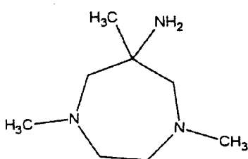
Compound 4
