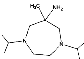
Compound 8
