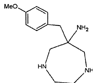
Compound 6
