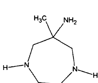
Compound 1
