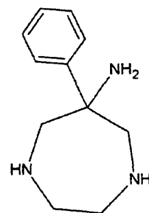
Compound 9
