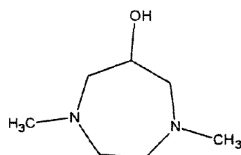
Compound 3
