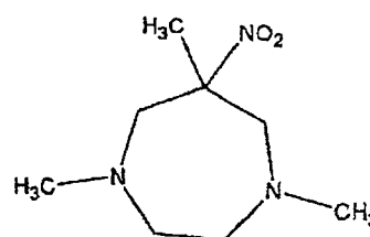
Compound Z
