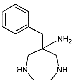
Compound 2
