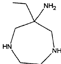
Compound 5
