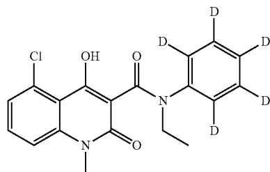
Compound 1
