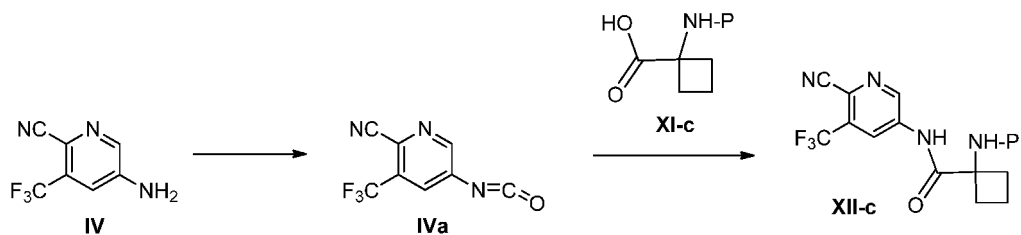
5-isocyanato-3-(trifluoromethyl)picolinonitrile
