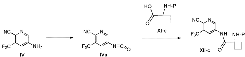
5-Isocyanato-3-(trifluormethyl)picolinonitril
