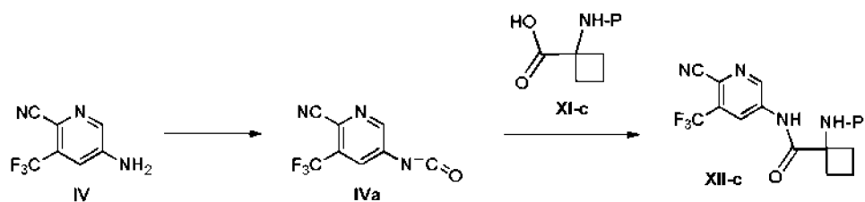
5-isocyanato-3-(trifluorométhyl)picolinonitrile
