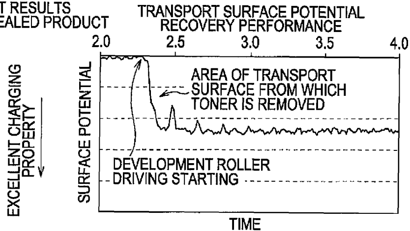
FIG. 9C 400°C ANNEALED PRODUCT
