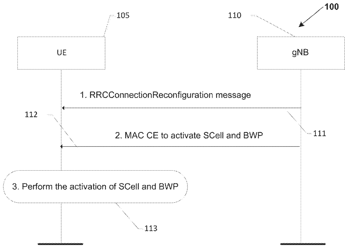
Example Activation of SCell and BWP
