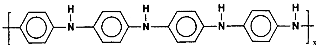
Leuco Emeraldine - Fully Reduced
