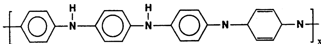
Emeraldine Base - Half Oxidized
