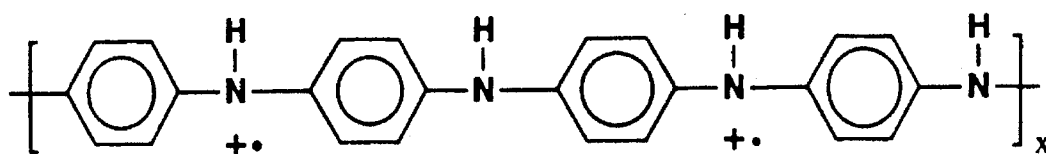
Emeraldine Salt - Half Oxidized
