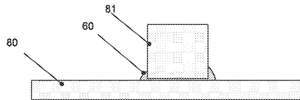
FIG. 31A - Adhesive dispense on composite substrate
