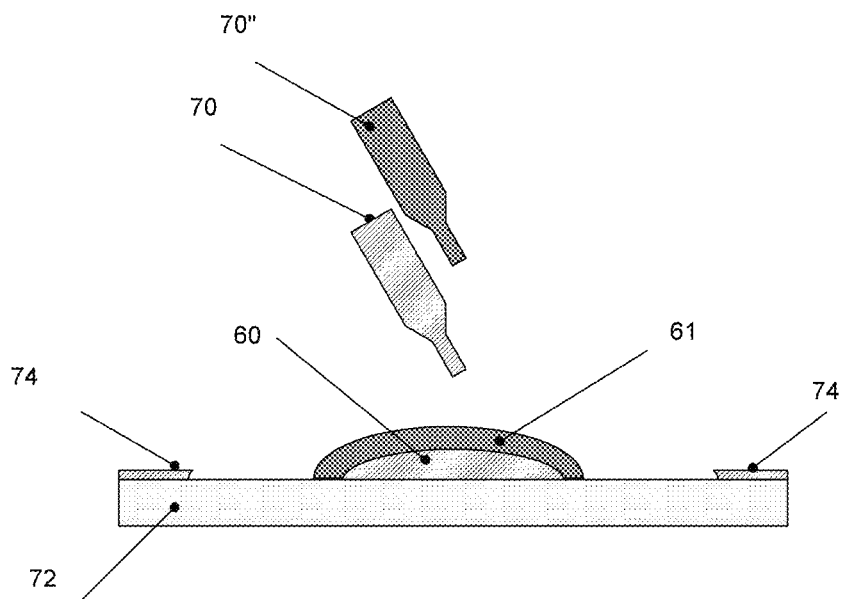
FIG. 33A - Dispensing of 2 adhesive beads
