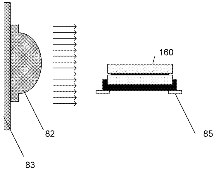
FIG. 37C The assemblies 160 are oriented in the same direction as the X-ray propagation (in the horizontal plane). Perspective along the direction of the conveyor system.
