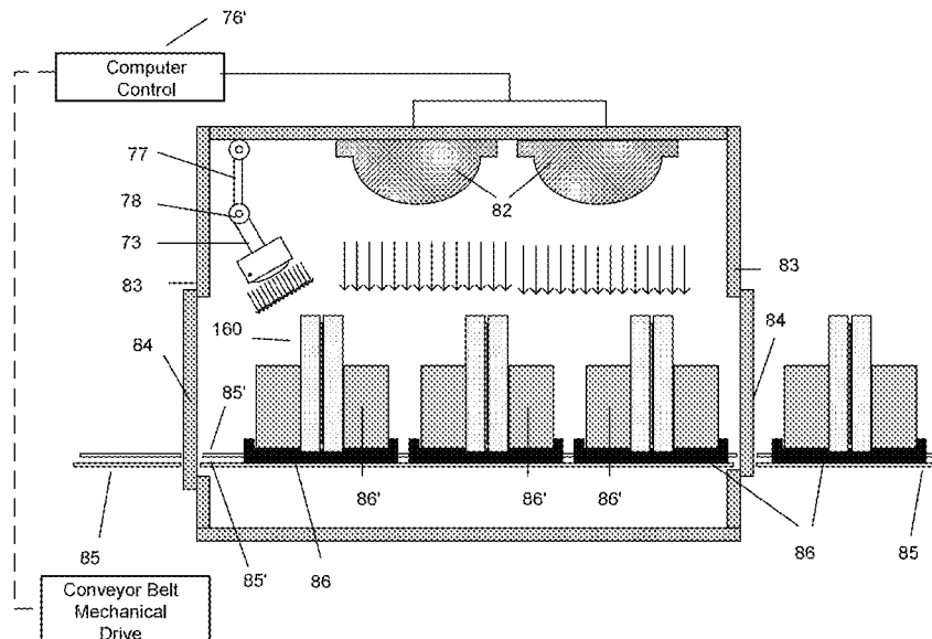
FIG. 37A The assemblies 160 are oriented in the same direction as the X-ray propagation in the vertical plane)
