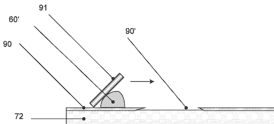
FIG. 30A - Alignment prior to screen printing
