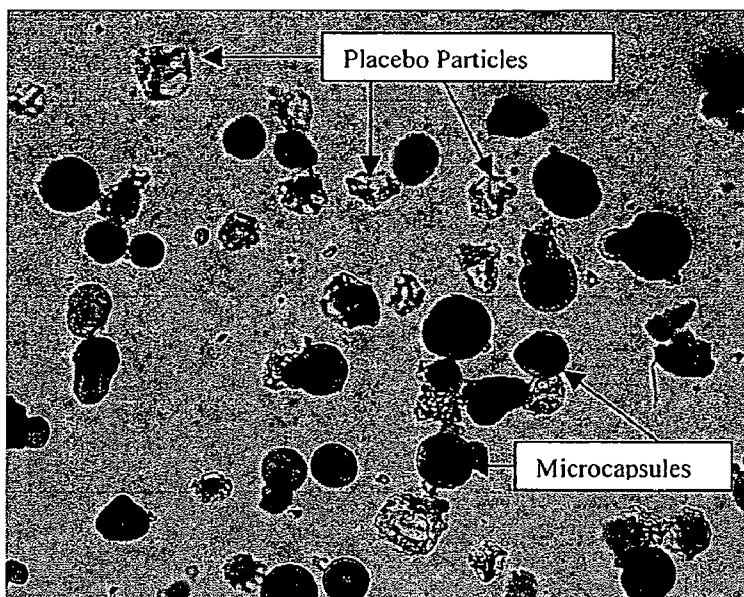
Microcapsules produced using conventional disk. (50X magnification)
