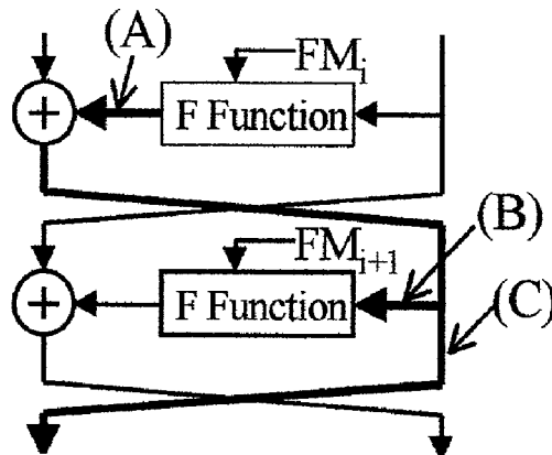
Propagation of Mask in Feistel Encryption
