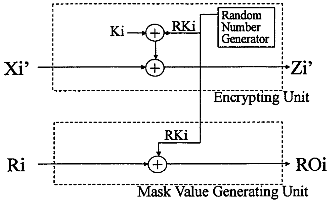
Key XOR in Random Mask Value Method
