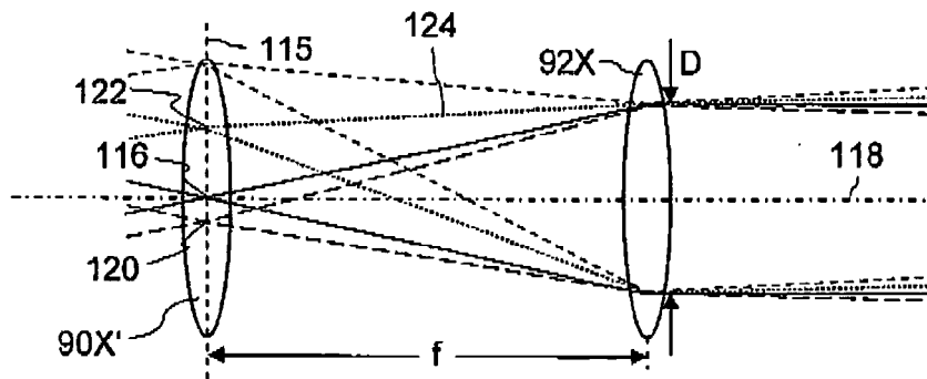
Fig. 8 (Prior Art)
