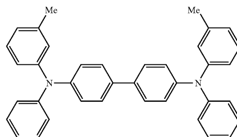
Compound 2
