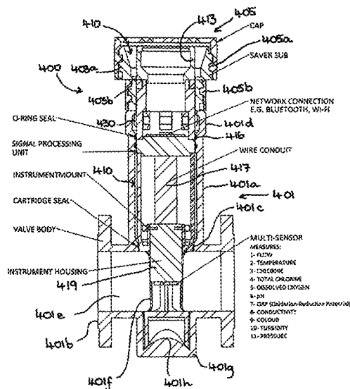
EXAMPLE OF INSTRUMENT SETUP - MULTI-SENSOR
