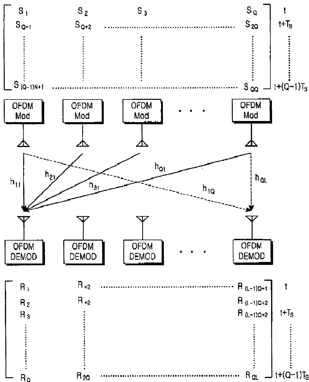
FIG. 4 (PRIOR ART)
