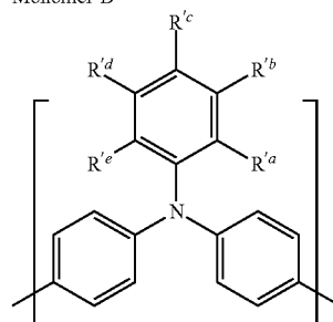
Monomer B
